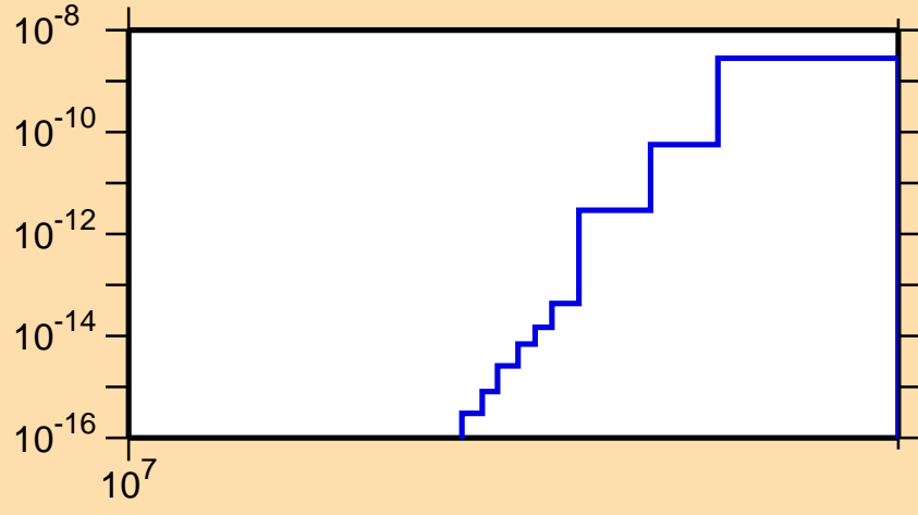
\sigma vs. E for ^{168}\text{Dy}(n,2n\alpha)
