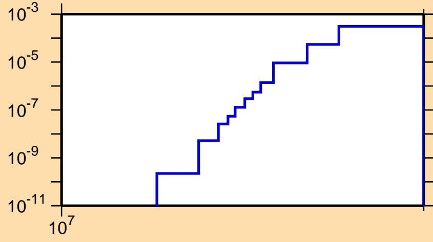
\sigma vs. E for ^{168}\text{Dy}(n,np)
