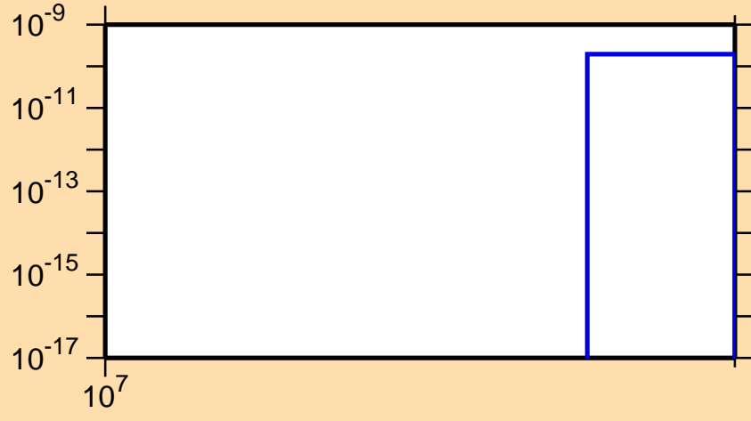
\sigma vs. E for ^{168}\text{Dy}(n,2np)
