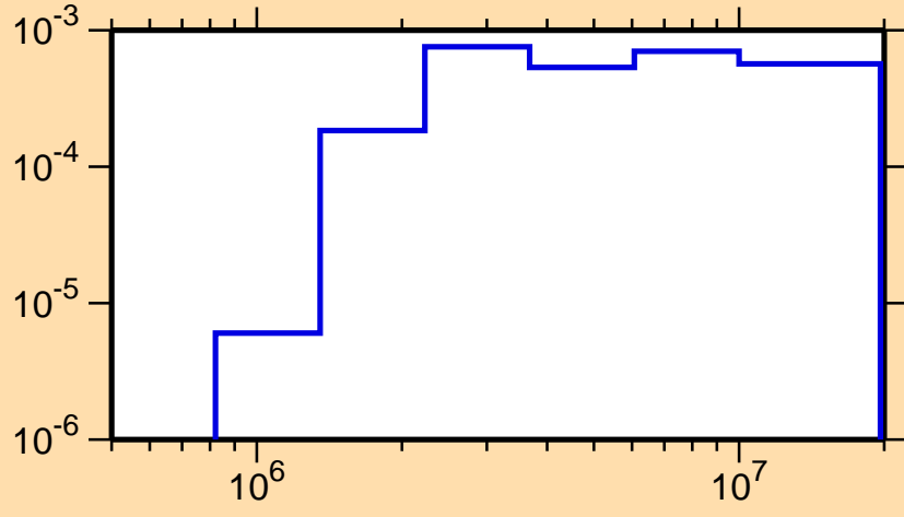
\sigma vs. E for ^{168}\text{Dy}(n,n_4)
