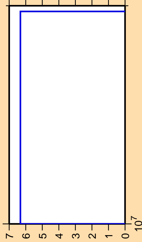
\Delta\sigma/\sigma vs. E for ^{168}\text{Dy}(n,2np)
