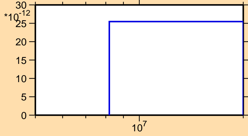
\sigma vs. E for ^{168}\text{Dy}(n,2n\alpha)
