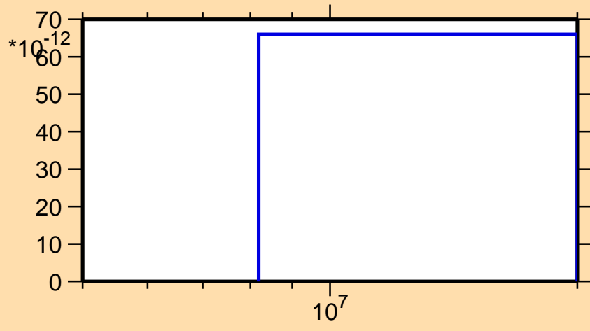
\sigma vs. E for ^{168}\text{Dy}(n,nd)
