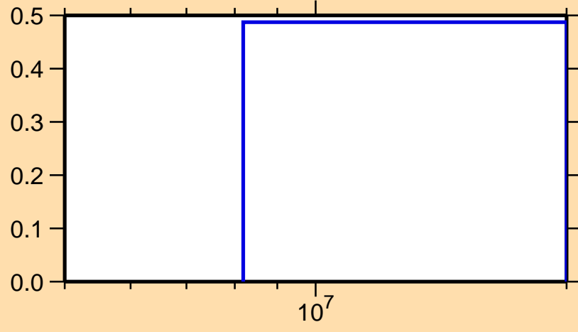
\sigma vs. E for ^{168}\text{Dy}(n,3n)
