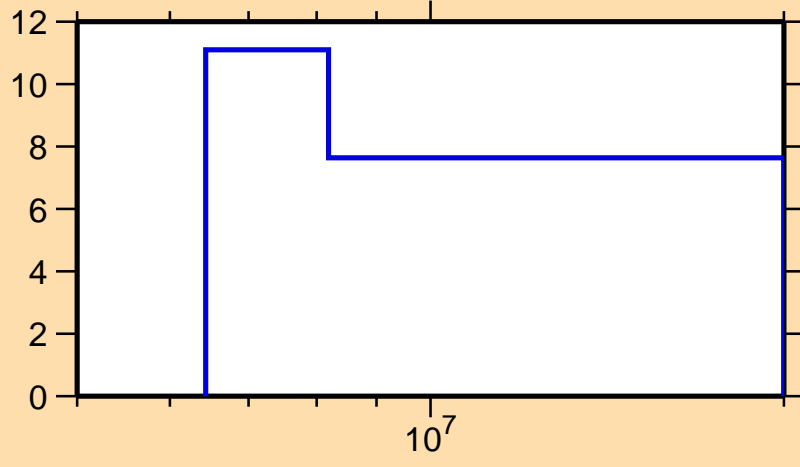
\Delta\sigma/\sigma vs. E for ^{168}\text{Dy}(n,\text{nonel.})
