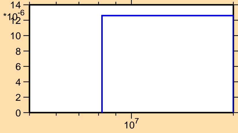
\sigma vs. E for ^{168}\text{Dy}(n,d)
