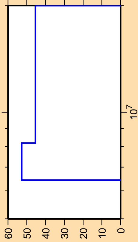
\Delta\sigma/\sigma vs. E for ^{168}\text{Dy}(n,n_1)
