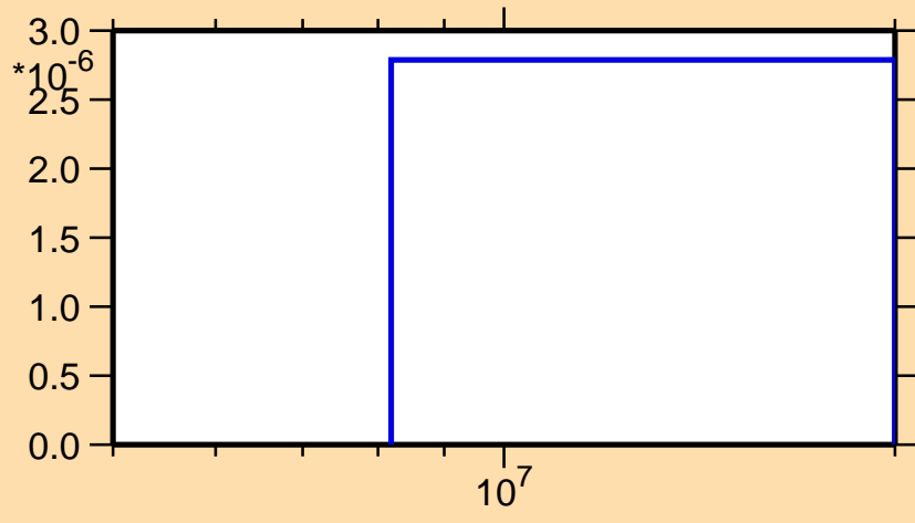
\sigma vs. E for ^{168}\text{Dy}(n,n\alpha)
