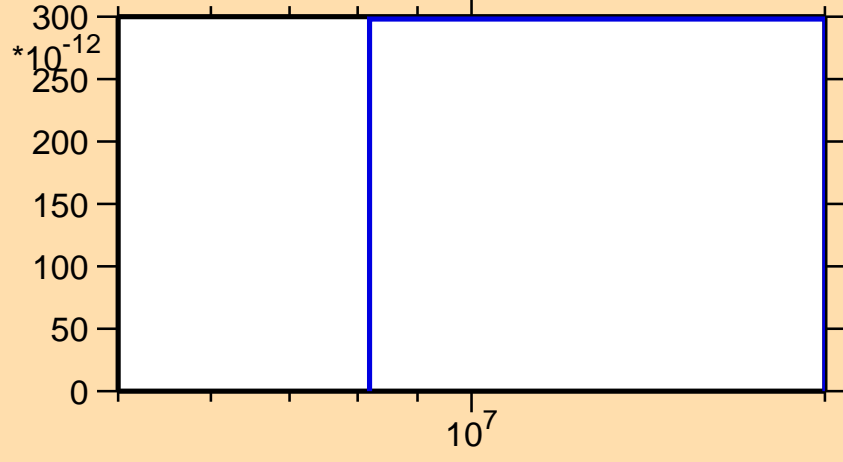
\sigma vs. E for ^{168}\text{Dy}(n,nt)
