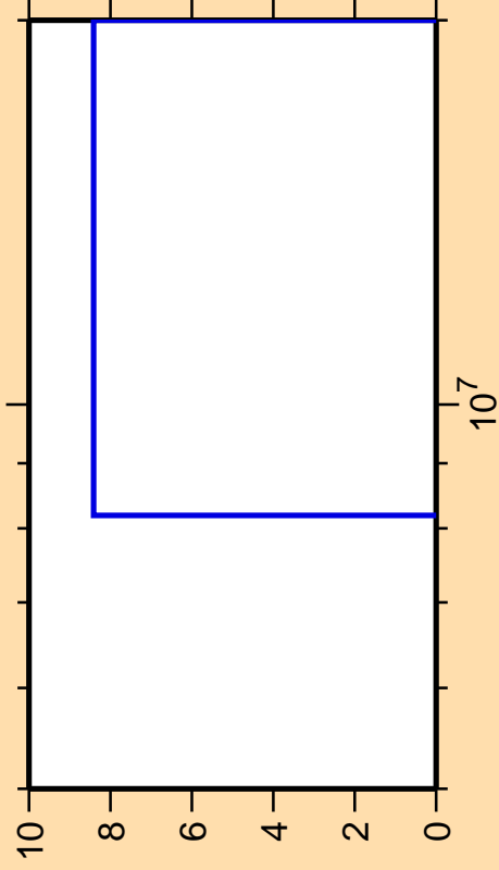
\Delta\sigma/\sigma vs. E for ^{168}\text{Dy}(n,2np)
