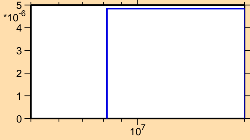
\sigma vs. E for ^{168}\text{Dy}(n,t)
