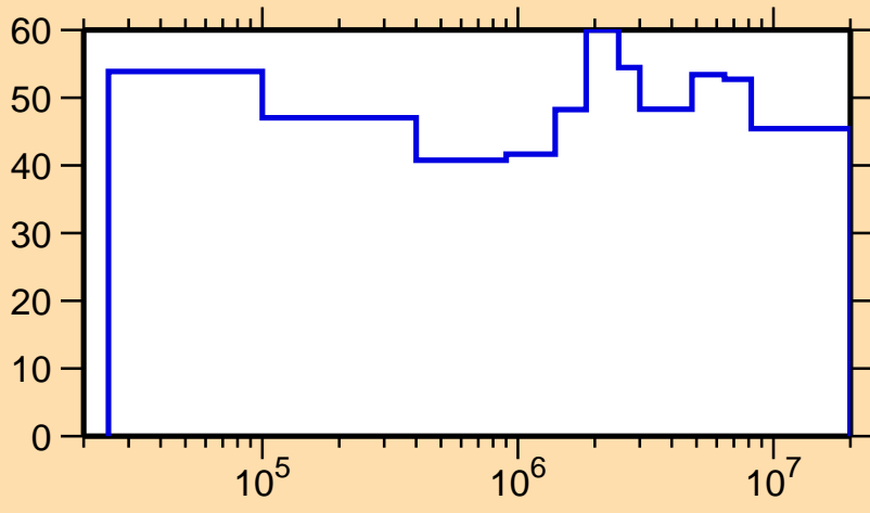
\Delta\sigma/\sigma vs. E for ^{168}\text{Dy}(n,n_1)
