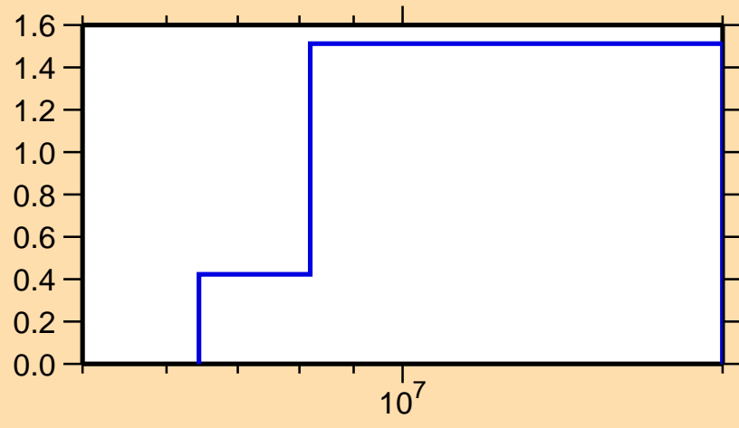
\sigma vs. E for ^{168}\text{Dy}(n,2n)
