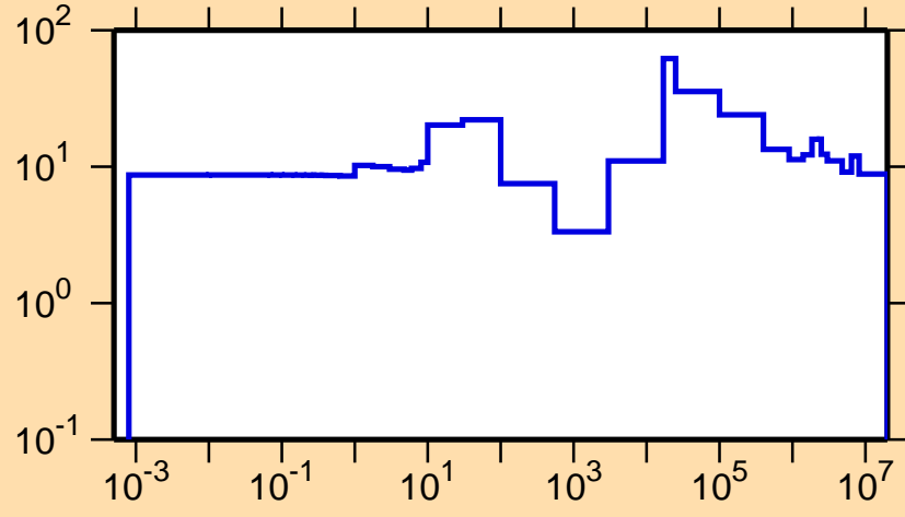
\Delta\sigma/\sigma vs. E for ^{168}\text{Dy}(n,\text{tot.})
