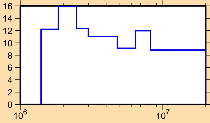
\Delta\sigma/\sigma vs. E for ^{168}\text{Dy}(n,\text{tot.})
