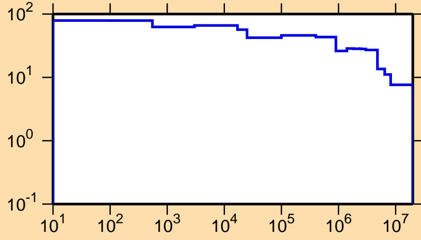
\Delta\sigma/\sigma vs. E for ^{168}\text{Dy}(n,\text{nonel.})
