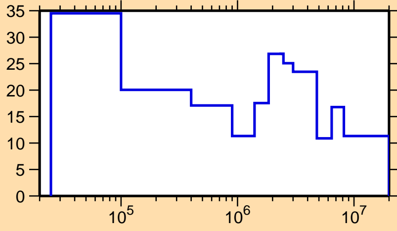
\Delta\sigma/\sigma vs. E for ^{168}\text{Dy}(n,\text{el.})
