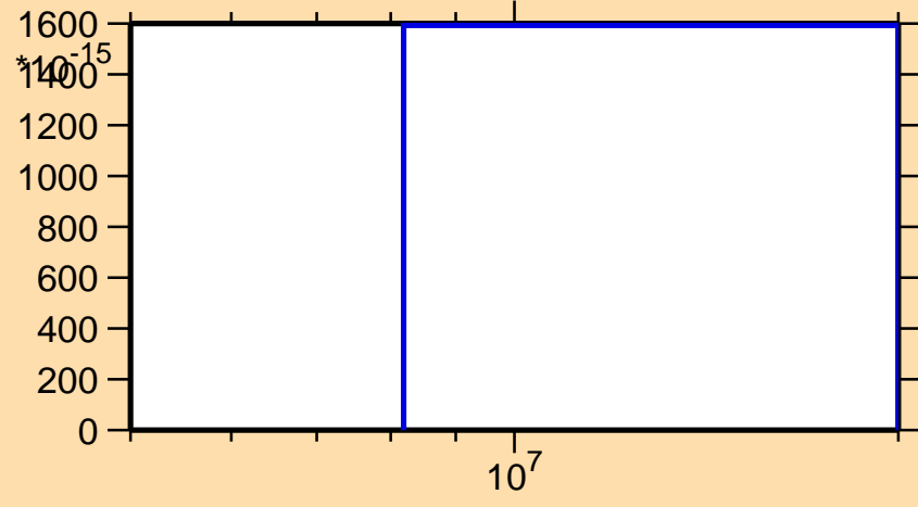
\sigma vs. E for ^{168}\text{Dy}(n,2np)
