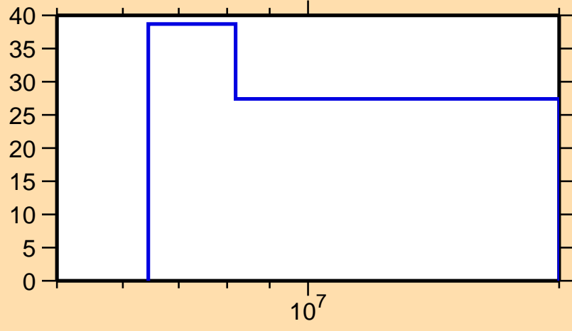
\Delta\sigma/\sigma vs. E for ^{168}\text{Dy}(n,2n)
