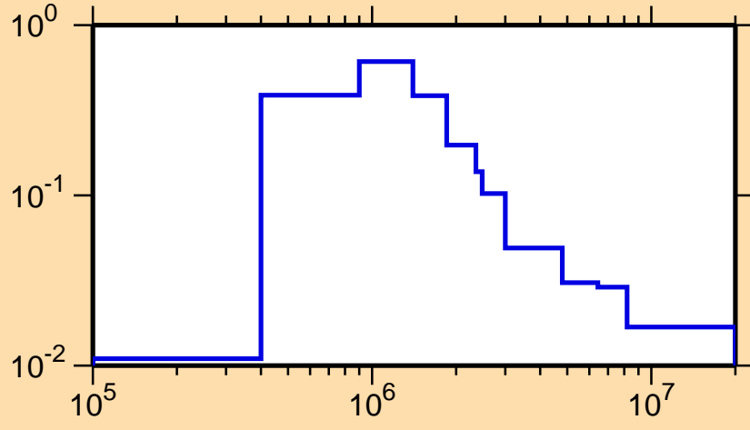
\sigma vs. E for ^{168}\text{Dy}(n,n_2)
