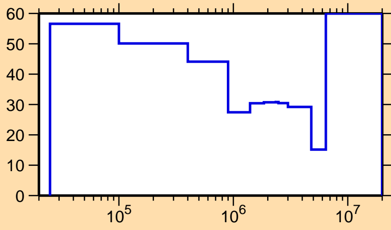
\Delta\sigma/\sigma vs. E for ^{168}\text{Dy}(n,\text{inel.})
