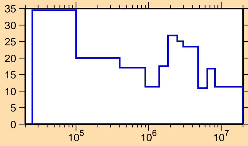
\Delta\sigma/\sigma vs. E for ^{168}\text{Dy}(n,\text{el.})
