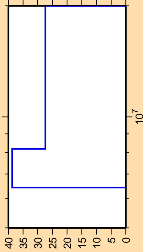
\Delta\sigma/\sigma vs. E for ^{168}\text{Dy}(n,2n)
