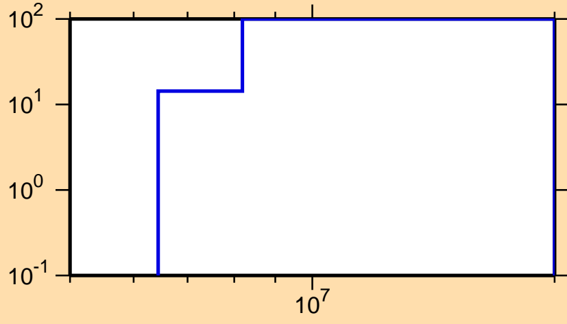
\Delta\sigma/\sigma vs. E for ^{168}\text{Dy}(n,p)
