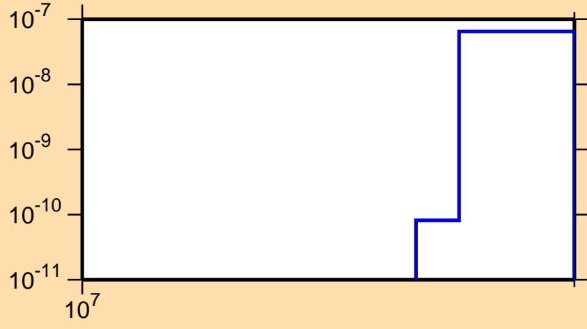
\sigma vs. E for ^{169}\text{Dy}(n,nt)
