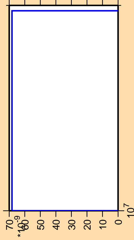
\Delta\sigma/\sigma vs. E for ^{169}\text{Dy} (mt 11)
