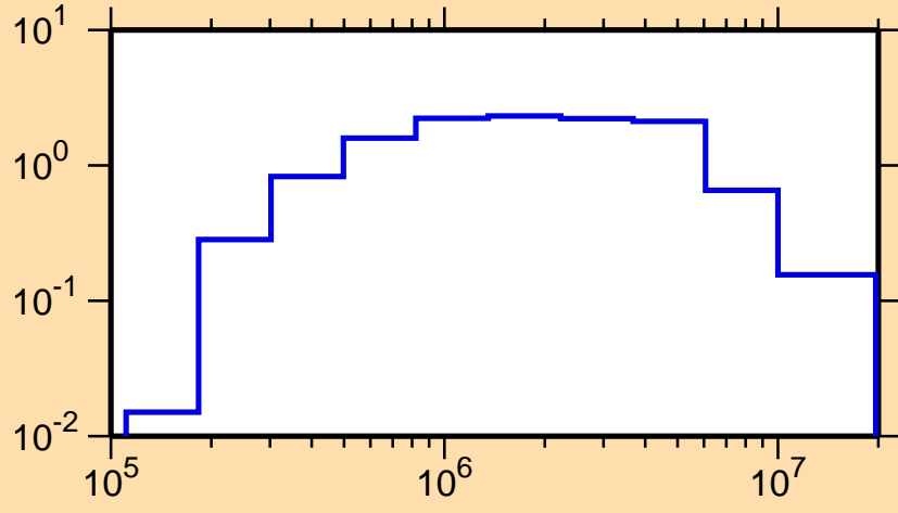
\sigma vs. E for ^{169}\text{Dy}(n,n\text{cont.})
