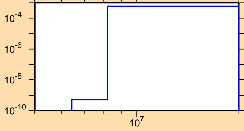
\sigma vs. E for ^{169}\text{Dy}(n,p)
