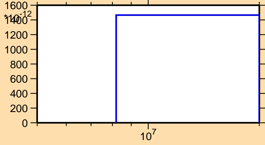
\sigma vs. E for ^{169}\text{Dy}(n,nd)
