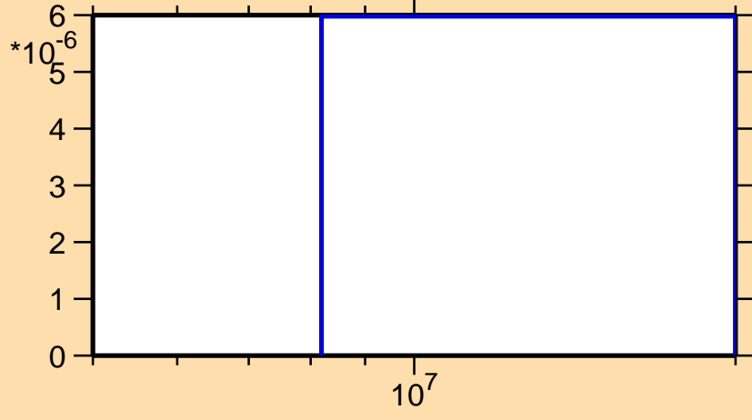
\sigma vs. E for ^{169}\text{Dy}(n,t)
