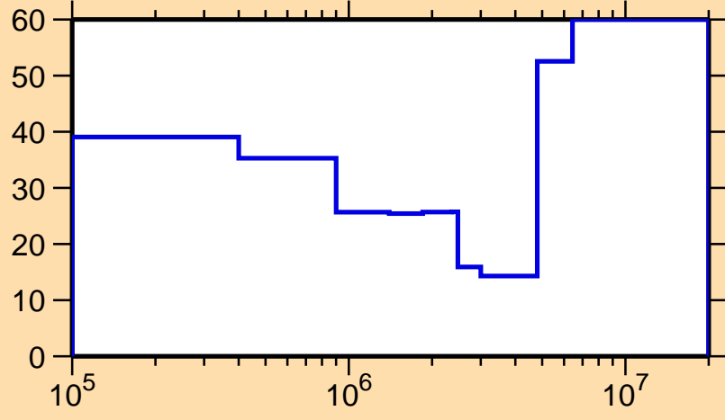
\Delta\sigma/\sigma vs. E for ^{169}\text{Dy}(n,\text{inel.})
