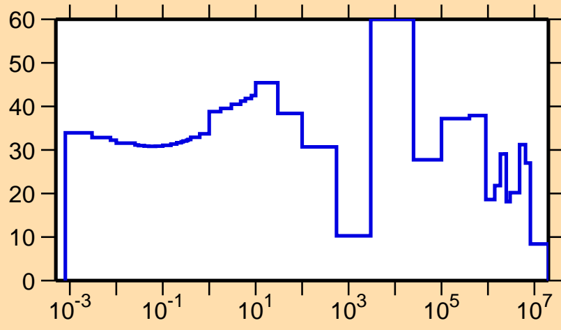
\Delta\sigma/\sigma vs. E for ^{169}\text{Dy}(n,\text{tot.})
