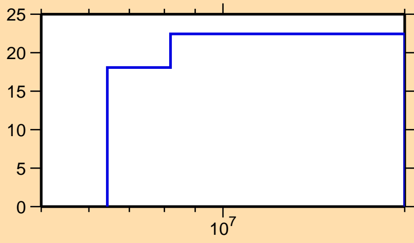
\Delta\sigma/\sigma vs. E for ^{169}\text{Dy}(n,2n)
