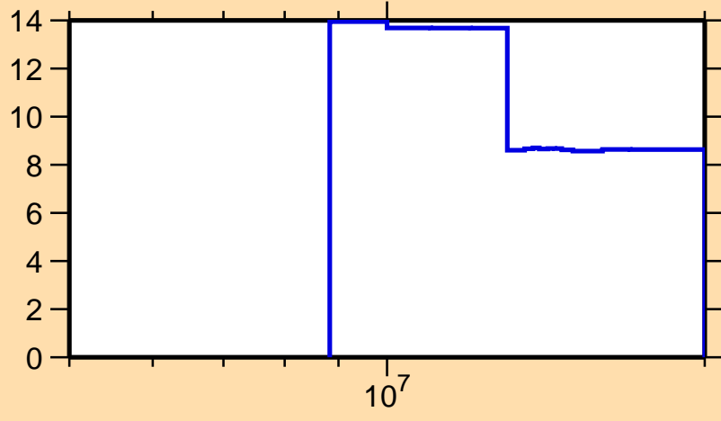
\Delta\sigma/\sigma vs. E for ^{170}\text{Dy}(n,el.)
