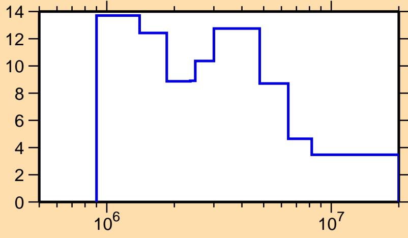
\Delta\sigma/\sigma vs. E for ^{170}\text{Dy}(n, tot.)
