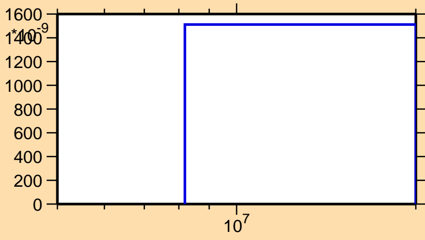
\sigma vs. E for ^{170}\text{Dy}(n,n\alpha)
