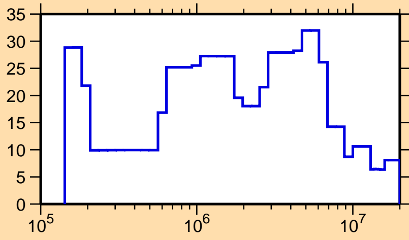
\Delta\sigma/\sigma vs. E for ^{171}\text{Dy}(n,\text{el.})
