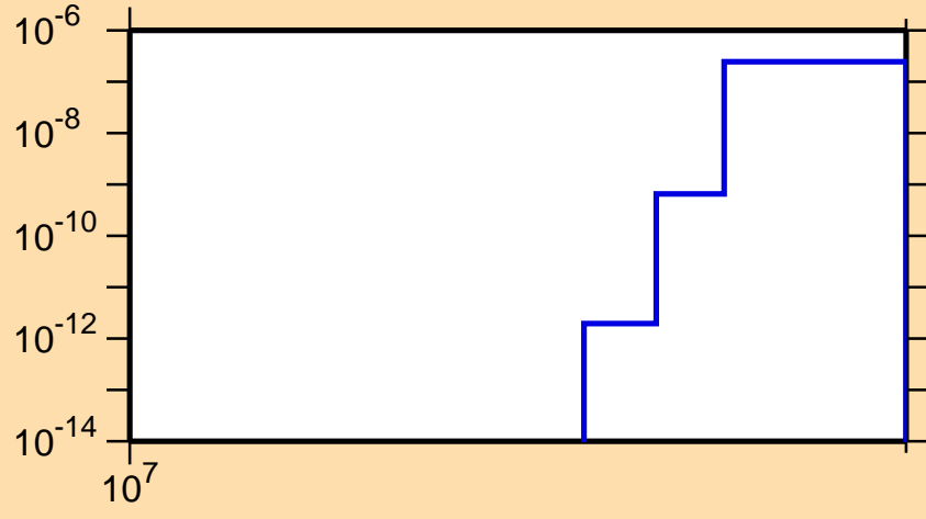
\sigma vs. E for ^{171}\text{Dy}(n,nt)
