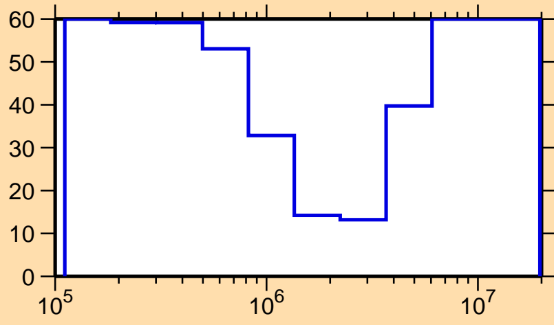
\Delta\sigma/\sigma vs. E for ^{171}\text{Dy}(n,\text{inel.})
