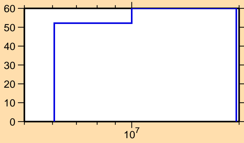
\Delta\sigma/\sigma vs. E for ^{171}\text{Dy}(n,p)
