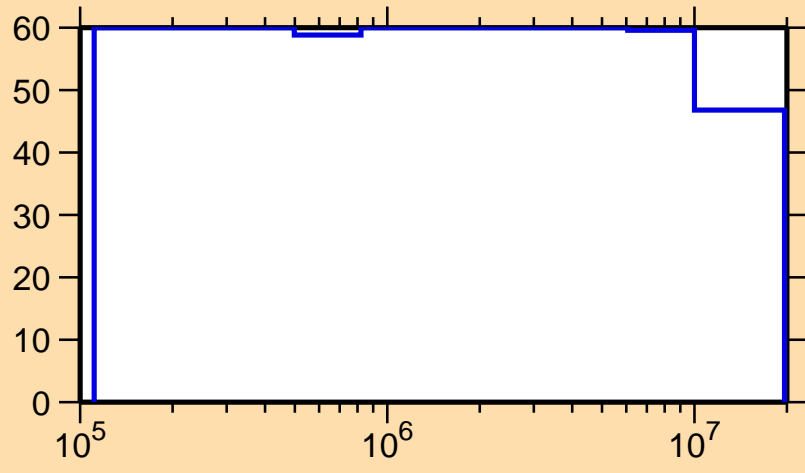
\Delta\sigma/\sigma vs. E for ^{171}\text{Dy}(n, n_1)
