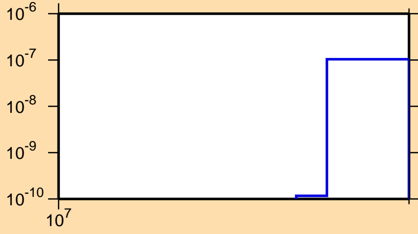
\sigma vs. E for ^{172}\text{Dy}(n,nt)
