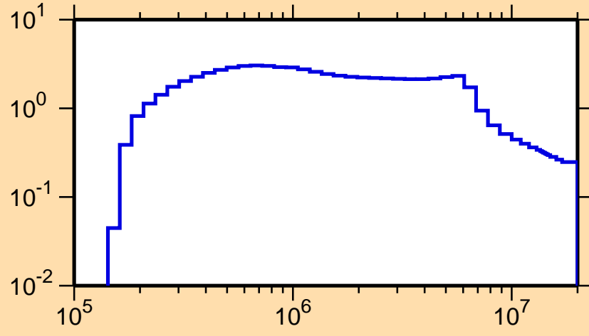
\sigma vs. E for ^{172}\text{Dy}(n,\text{inel.})
