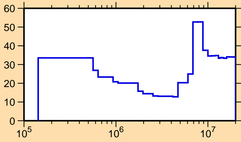
\Delta\sigma/\sigma vs. E for ^{172}\text{Dy}(n,\text{inel.})
