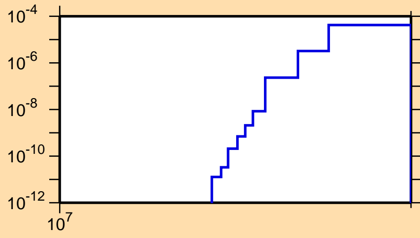
\sigma vs. E for ^{172}\text{Dy}(n,np)
