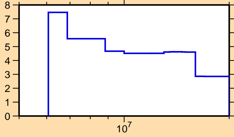
\Delta\sigma/\sigma vs. E for ^{172}\text{Dy}(n,\text{nonel.})
