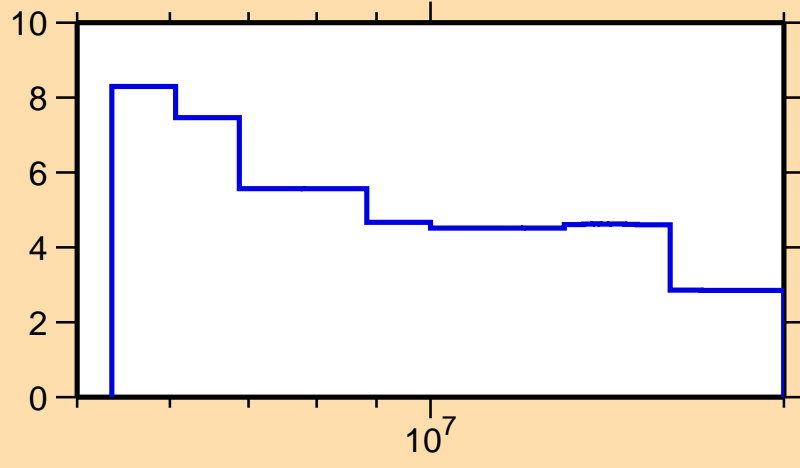
\Delta\sigma/\sigma vs. E for ^{172}\text{Dy}(n,\text{nonel.})
