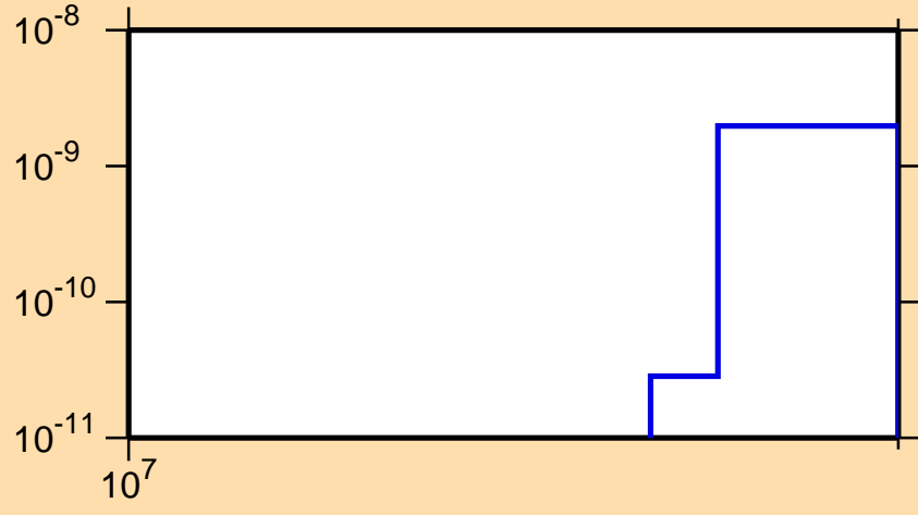
\sigma vs. E for ^{172}\text{Dy}(n,2n\alpha)
