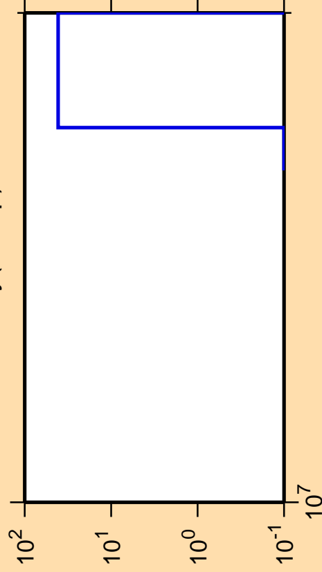
\Delta\sigma/\sigma vs. E for ^{172}\text{Dy}(n,2np)
