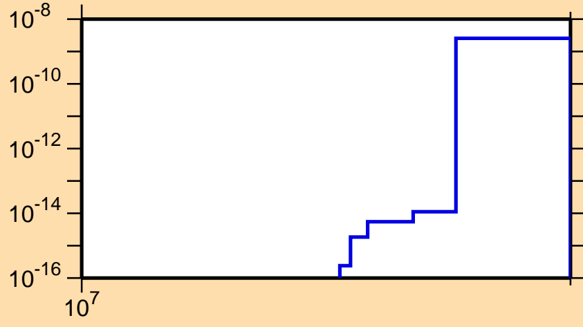
\sigma vs. E for ^{172}\text{Dy}(n,nd)
