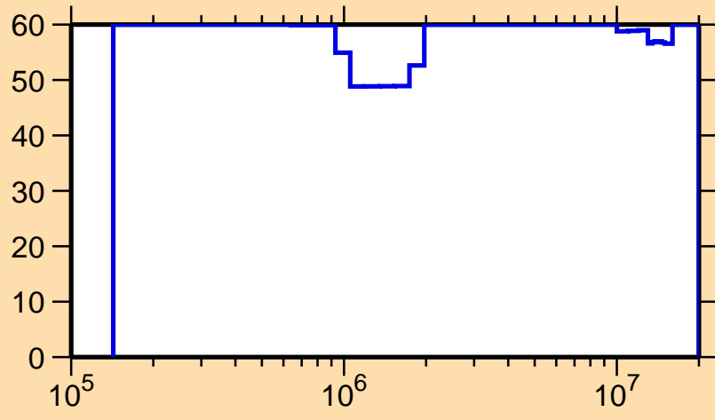
\Delta\sigma/\sigma vs. E for ^{172}\text{Dy}(n,n_1)
