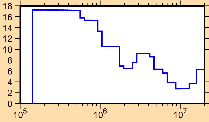
\Delta\sigma/\sigma vs. E for ^{172}\text{Dy}(n,\text{tot.})
