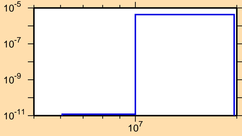
\sigma vs. E for ^{172}\text{Dy}(n,\alpha)
