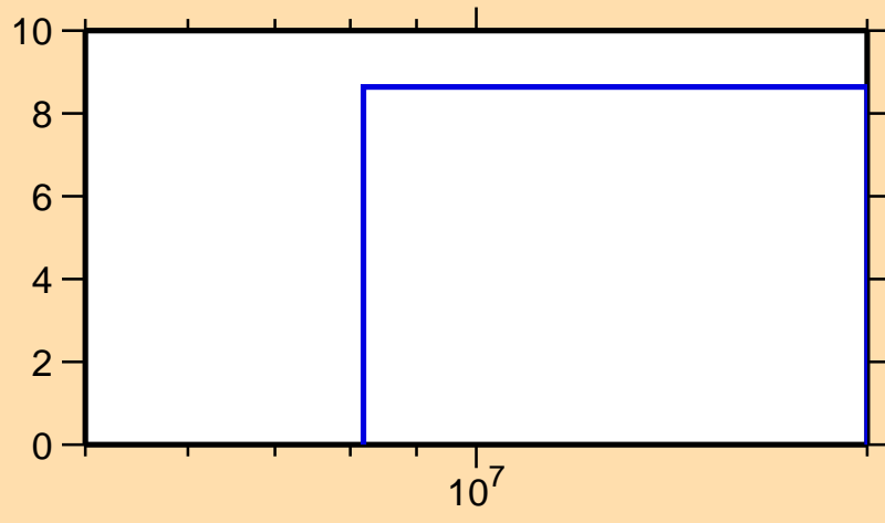
\Delta\sigma/\sigma vs. E for ^{172}\text{Dy}(n,el.)
