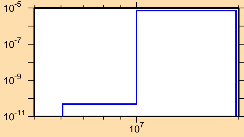
\sigma vs. E for ^{173}\text{Dy}(n,\alpha)
