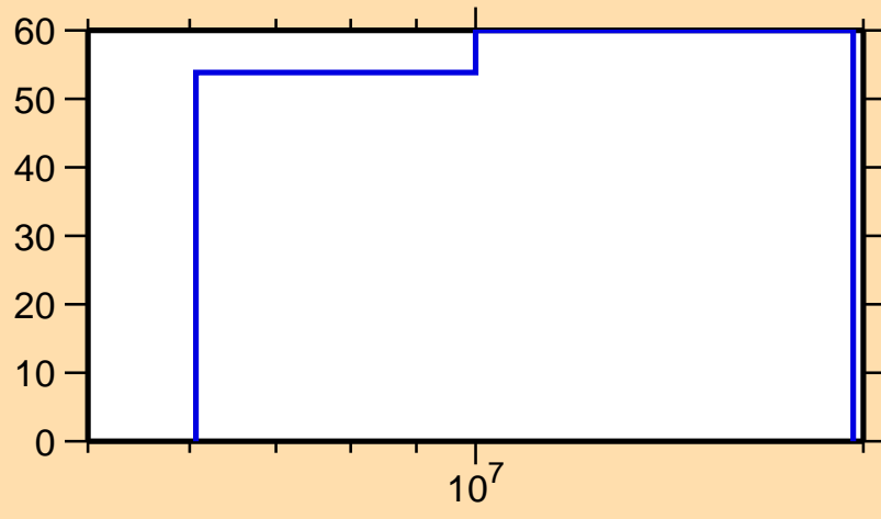
\Delta\sigma/\sigma vs. E for ^{173}\text{Dy}(n,p)
