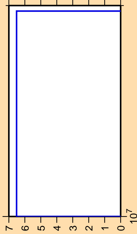
\Delta\sigma/\sigma vs. E for ^{173}\text{Dy}(n,2np)
