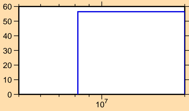
\Delta\sigma/\sigma vs. E for ^{173}\text{Dy}(n,ncont.)
