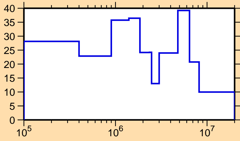
\Delta\sigma/\sigma vs. E for ^{173}\text{Dy}(n,el.)
