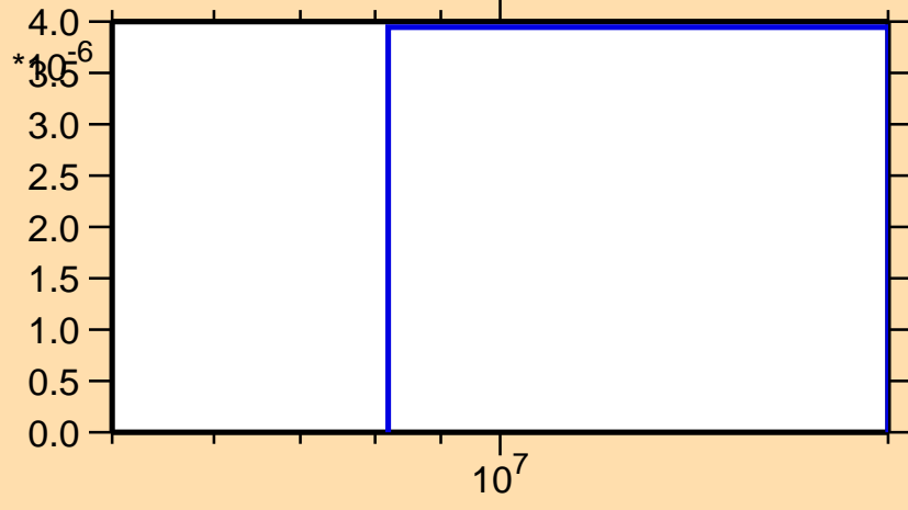
\sigma vs. E for ^{173}\text{Dy}(n,t)
