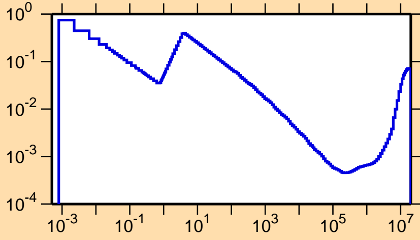
\sigma vs. E for ^{148}\text{Er}(n,\alpha)
