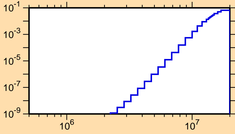
\sigma vs. E for ^{148}\text{Er}(n,p\alpha)
