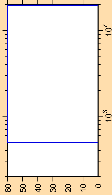
\Delta\sigma/\sigma vs. E for ^{148}\text{Er}(n,n_1)
