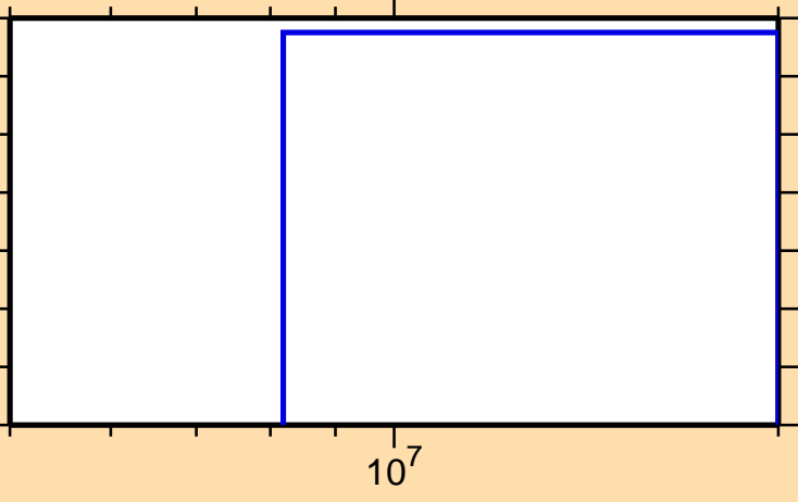
\sigma vs. E for ^{148}\text{Er}(\text{mt } 45)
