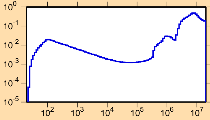
\sigma vs. E for ^{149}\text{Er}(n,\text{inel.})
