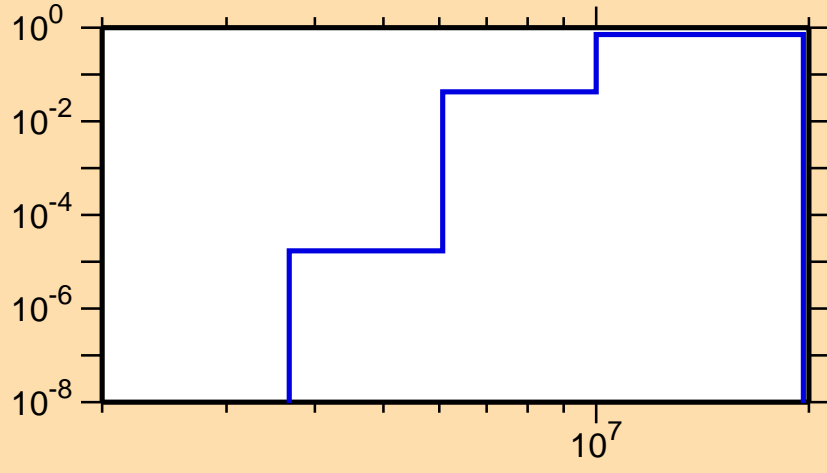
\sigma vs. E for ^{149}\text{Er}(n,np)
