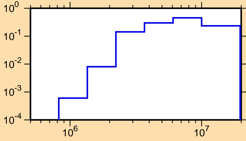
\sigma vs. E for ^{149}\text{Er}(n,n\text{cont.})
