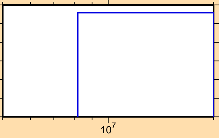
\sigma vs. E for ^{149}\text{Er}(n,2n)
