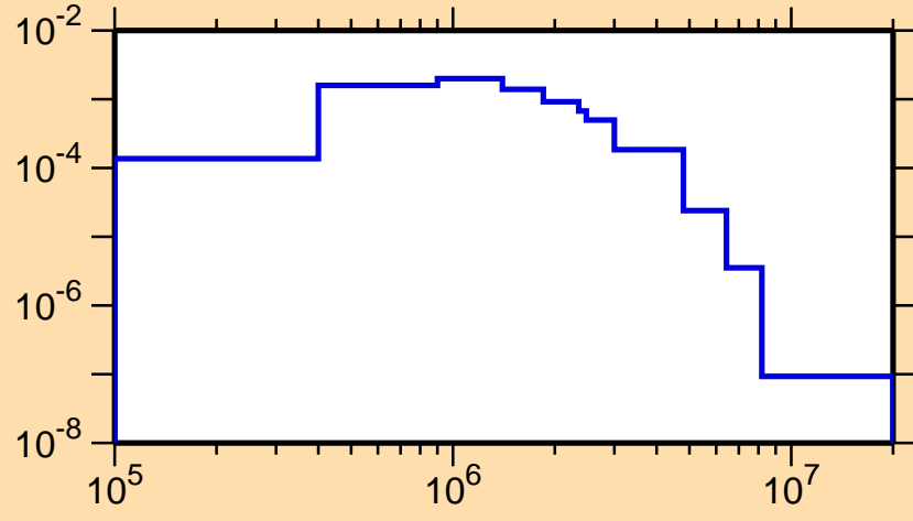
\sigma vs. E for ^{149}\text{Er}(n,n_3)
