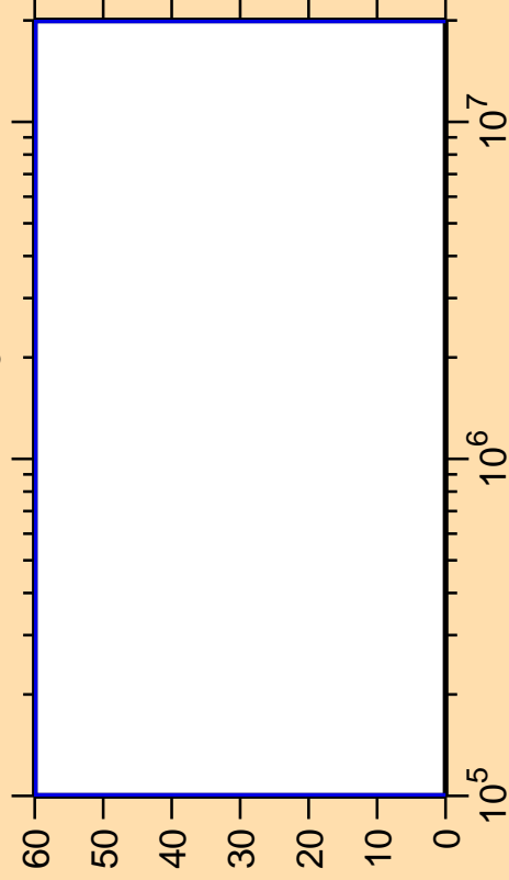
\Delta\sigma/\sigma vs. E for ^{149}\text{Er}(n,n_3)
