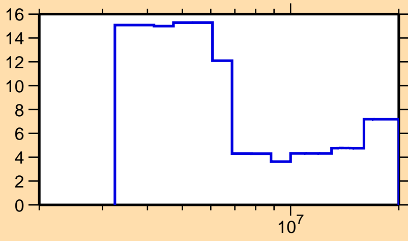
\Delta\sigma/\sigma vs. E for ^{152}\text{Er}(n, el.)
