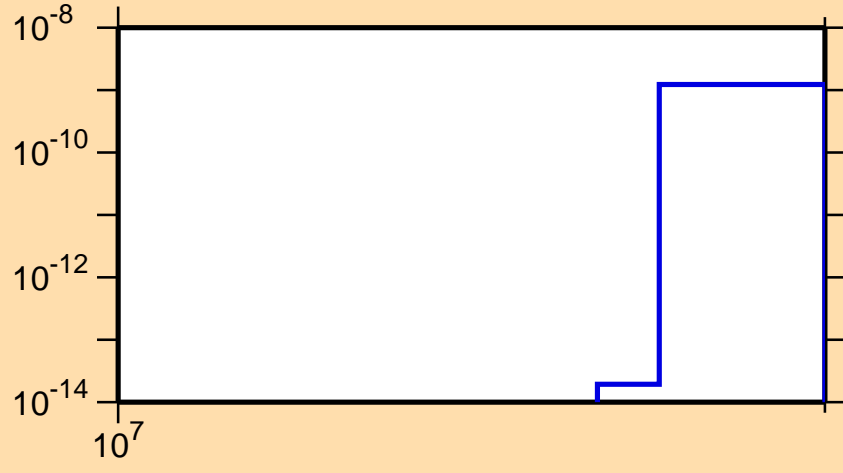
\sigma vs. E for ^{152}\text{Er}(n,nt)
