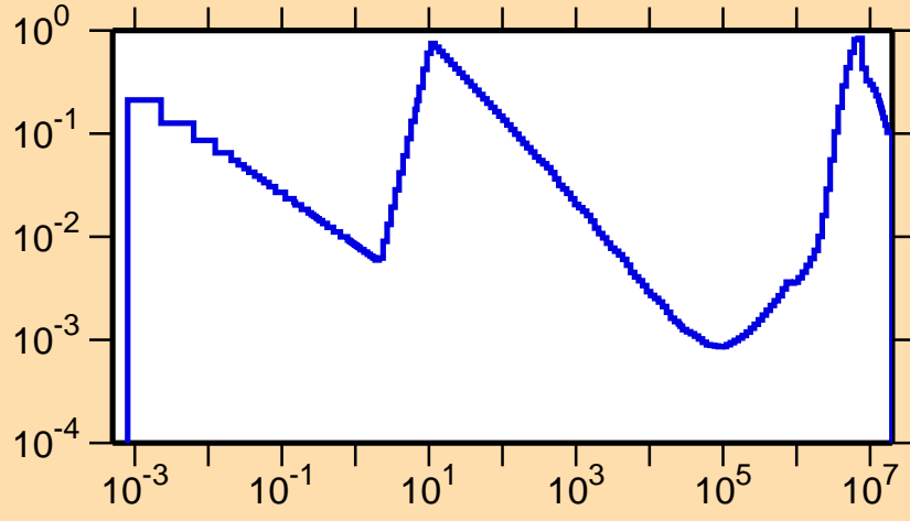
\sigma vs. E for ^{152}\text{Er}(n,p)
