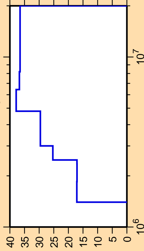
\Delta\sigma/\sigma vs. E for ^{152}\text{Er}(n,n_3)
