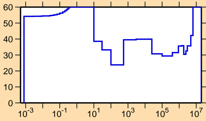
\Delta\sigma/\sigma vs. E for ^{152}\text{Er}(n,\gamma)
