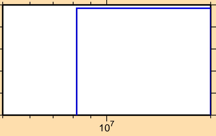
\sigma vs. E for ^{152}\text{Er}(n,t)
