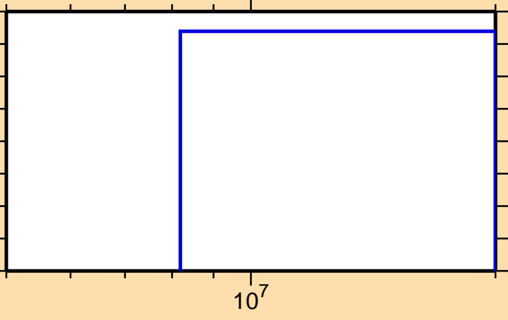
\sigma vs. E for ^{152}\text{Er}(n,\text{nd})
