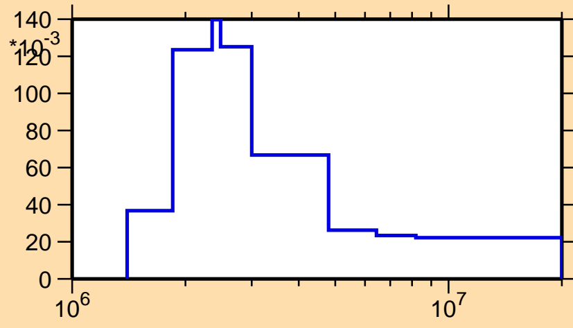
\sigma vs. E for ^{152}\text{Er}(n,n_3)
