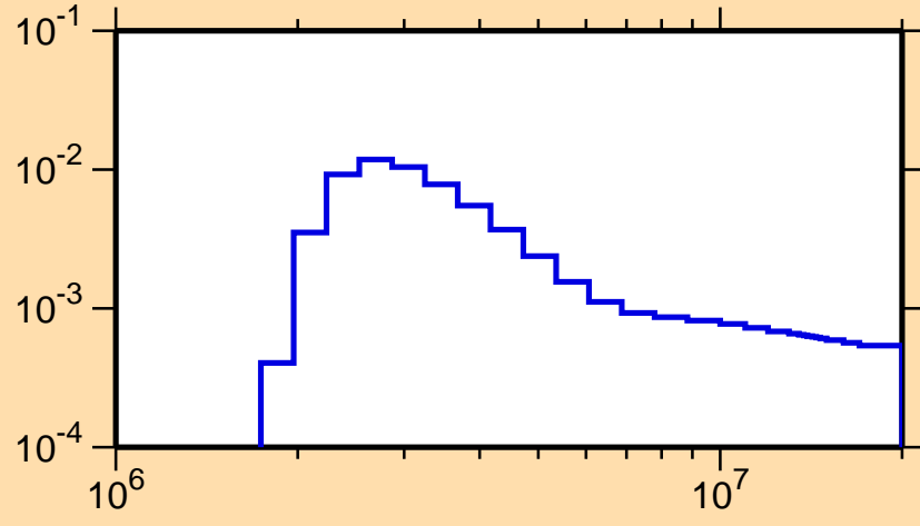
\sigma vs. E for ^{154}\text{Er}(n,n_3)
