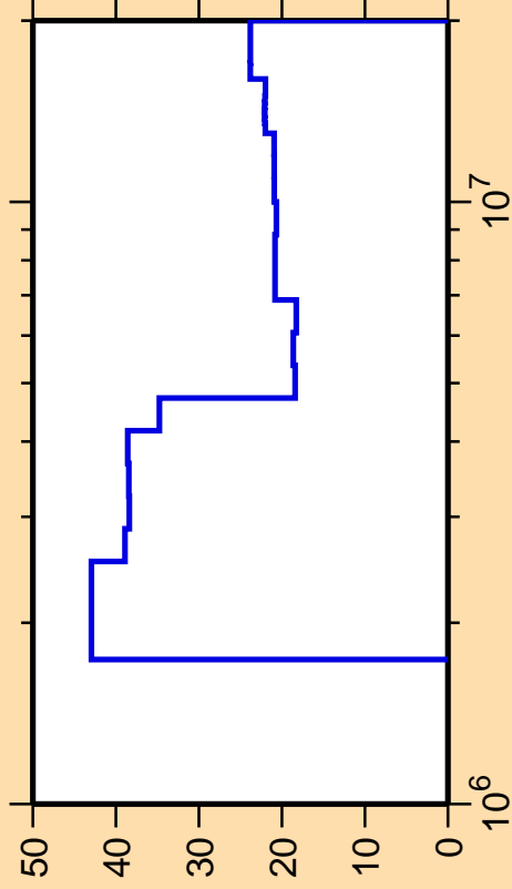
\Delta\sigma/\sigma vs. E for ^{154}\text{Er}(n,n_3)
