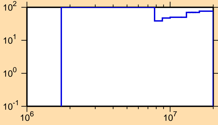
\Delta\sigma/\sigma vs. E for ^{154}\text{Er}(n,n\text{cont.})
