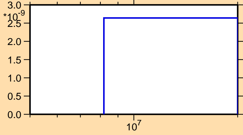
\sigma vs. E for ^{154}\text{Er}(n,\text{nd})
