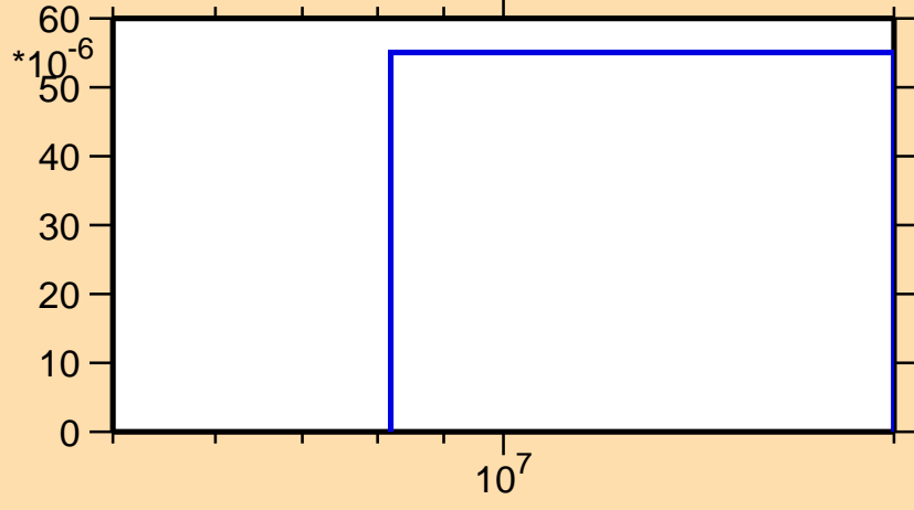
\sigma vs. E for ^{154}\text{Er}(n,t)
