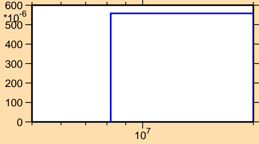
\sigma vs. E for ^{154}\text{Er}(n,2n\alpha)
