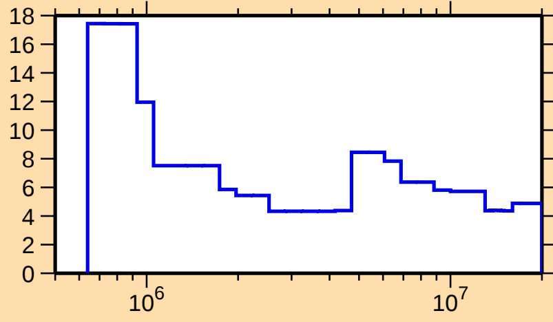
\Delta\sigma/\sigma vs. E for ^{161}\text{Er}(n,\text{nonel.})
