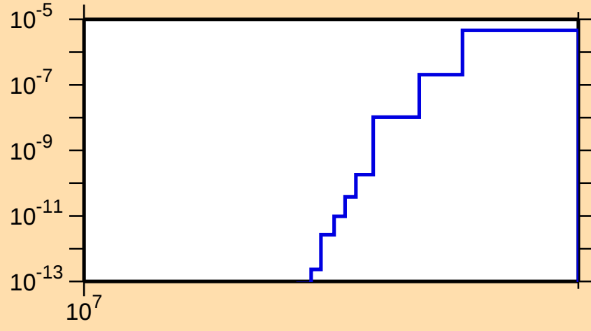
\sigma vs. E for ^{161}\text{Er}(n,\text{nd})
