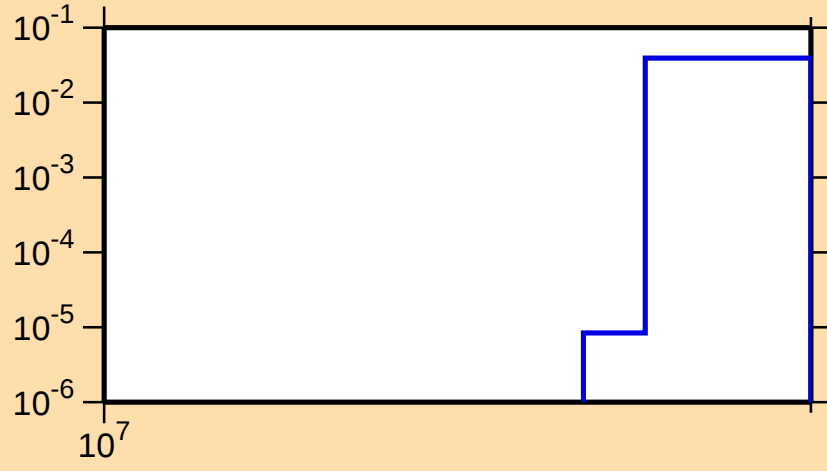
\sigma vs. E for ^{161}\text{Er}(n,3n)
