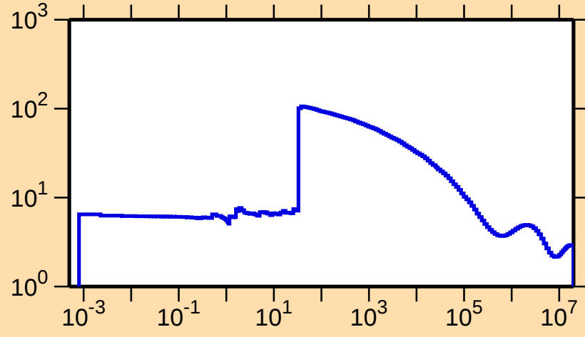
\sigma vs. E for ^{161}\text{Er}(n,\text{el.})
