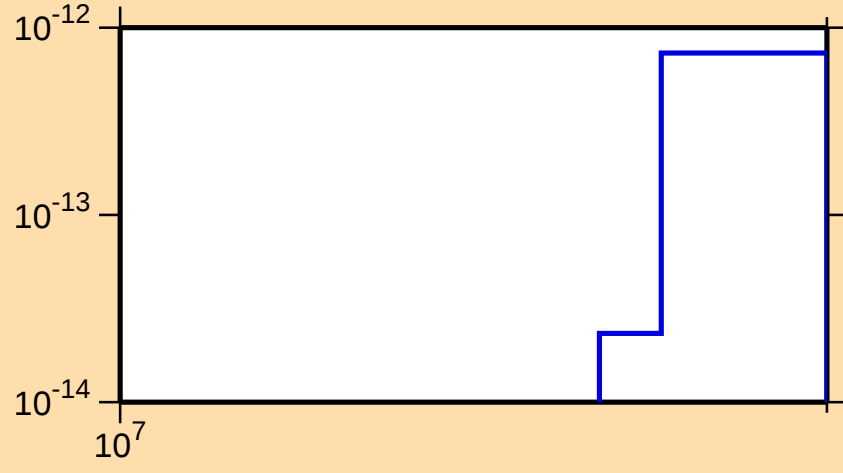
\sigma vs. E for ^{161}\text{Er} (mt 45)
