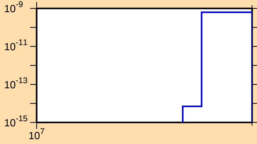
\sigma vs. E for ^{161}\text{Er}(n,\text{nt})
