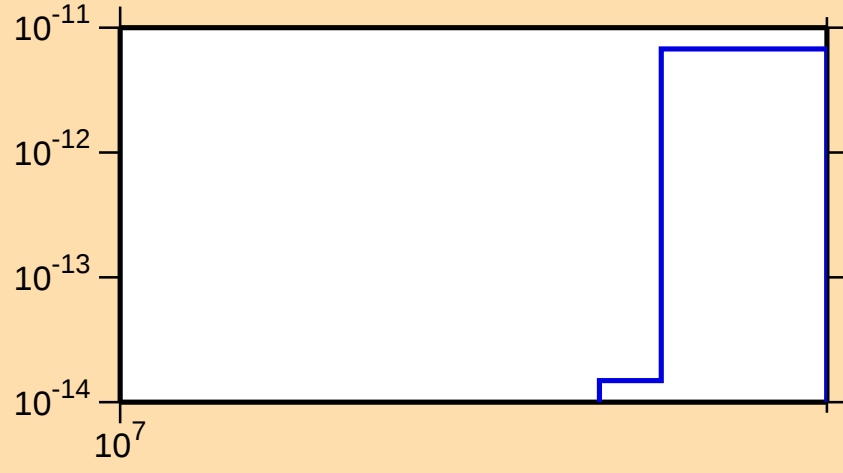
\sigma vs. E for ^{161}\text{Er}(\text{mt 34})
