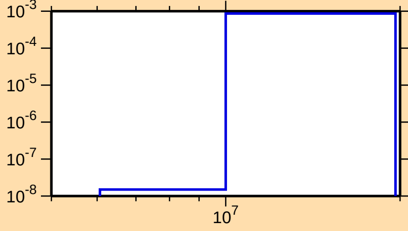
\sigma vs. E for ^{162}\text{Er}(n,d)
