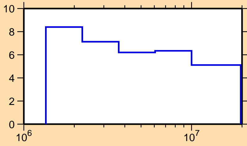
\Delta\sigma/\sigma vs. E for ^{168}\text{Er}(n,\text{nonel.})
