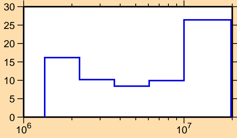
\Delta\sigma/\sigma vs. E for ^{168}\text{Er}(n,n\text{cont.})
