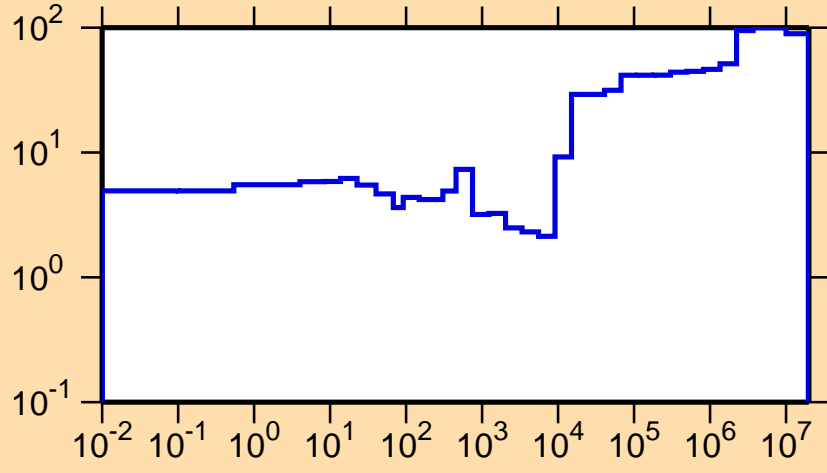
\Delta\sigma/\sigma vs. E for ^{168}\text{Er}(n,\gamma)
