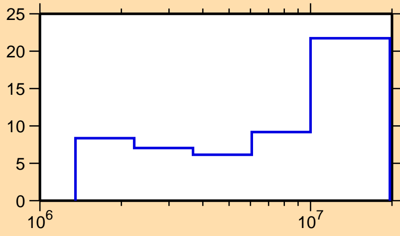
\Delta\sigma/\sigma vs. E for ^{168}\text{Er}(n,\text{inel.})
