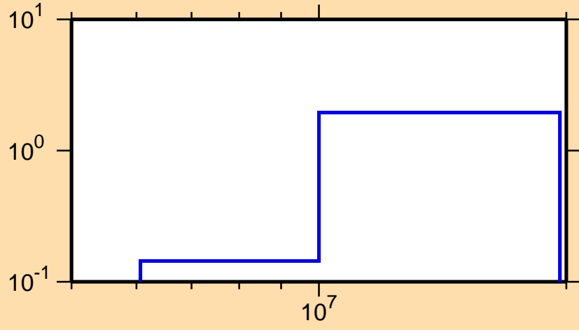
\sigma vs. E for ^{168}\text{Er}(n,2n)
