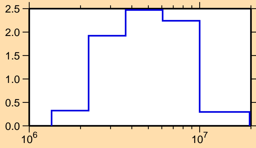
\sigma vs. E for ^{168}\text{Er}(n,n\text{cont.})
