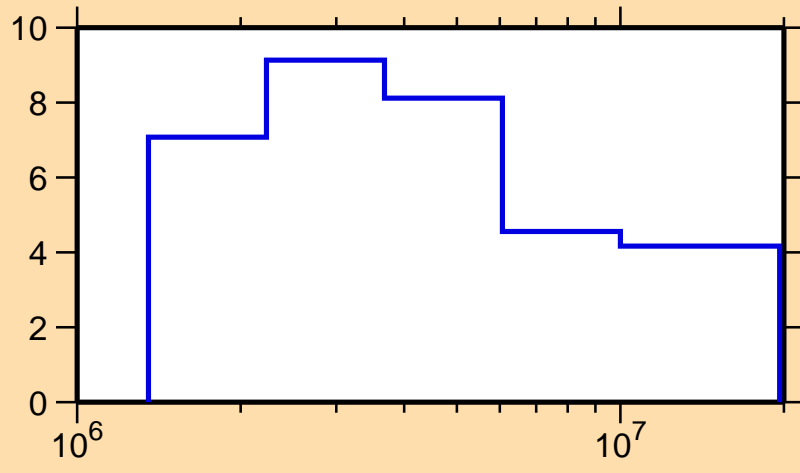
\Delta\sigma/\sigma vs. E for ^{168}\text{Er}(n,\text{tot.})
