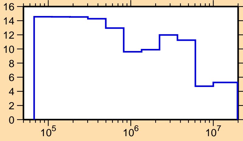
\Delta\sigma/\sigma vs. E for ^{168}\text{Er}(n,\text{el.})
