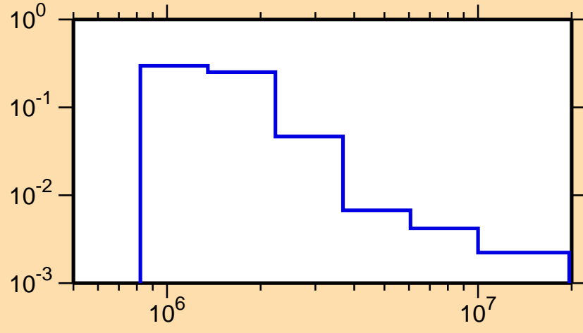
\sigma vs. E for ^{168}\text{Er}(n,n_4)
