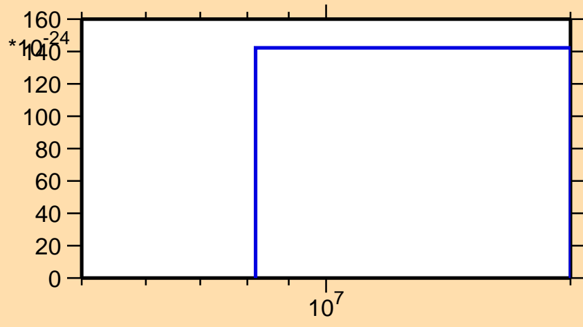
\sigma vs. E for ^{168}\text{Er}(\text{mt } 11)
