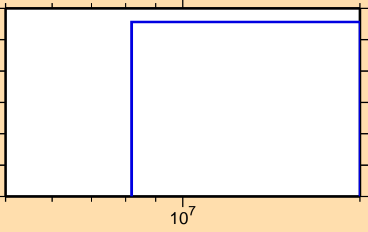
\sigma vs. E for ^{168}\text{Er}(n,3n)
