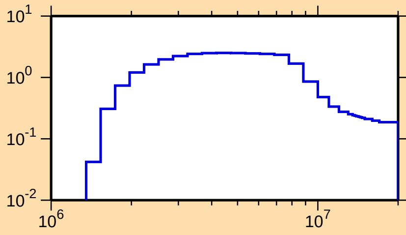
\sigma vs. E for ^{170}\text{Er}(n,n\text{cont.})
