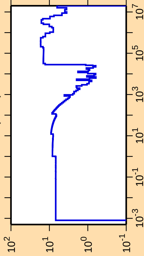
\Delta\sigma/\sigma vs. E for ^{170}\text{Er}(n,\text{el.})
