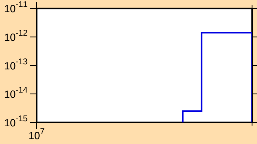
\sigma vs. E for ^{170}\text{Er}(n,\text{He3})
