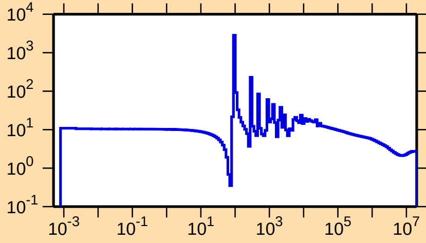
\sigma vs. E for ^{170}\text{Er}(n,\text{el.})
