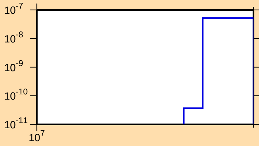
\sigma vs. E for ^{170}\text{Er}(n,\text{nd})
