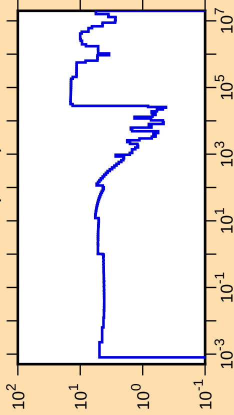
\Delta\sigma/\sigma vs. E for ^{170}\text{Er}(n,\text{tot.})
