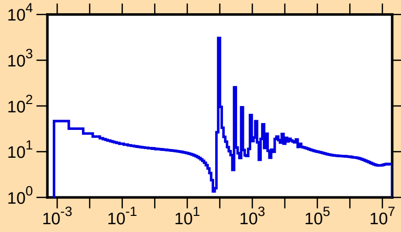
\sigma vs. E for ^{170}\text{Er}(n,\text{tot.})
