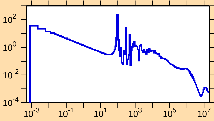
\sigma vs. E for ^{170}\text{Er}(n,\gamma)
