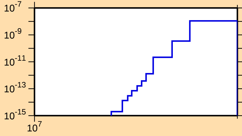
\sigma vs. E for ^{172}\text{Er}(n,2n\alpha)
