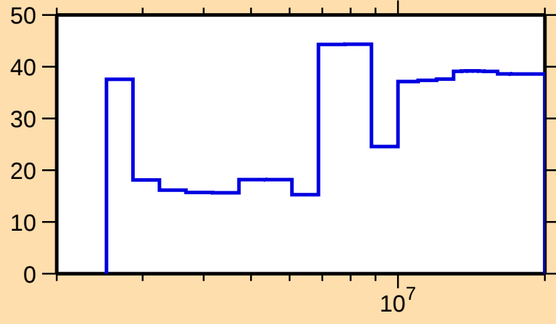
\Delta\sigma/\sigma vs. E for ^{172}\text{Er}(n,n\text{cont.})
