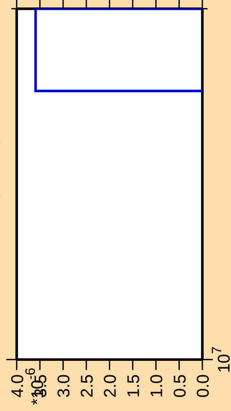
\Delta\sigma/\sigma vs. E for ^{172}\text{Er}(\text{mt 11})
