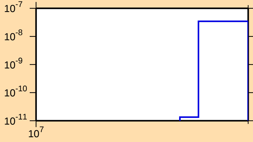
\sigma vs. E for ^{172}\text{Er}(n,\text{nd})
