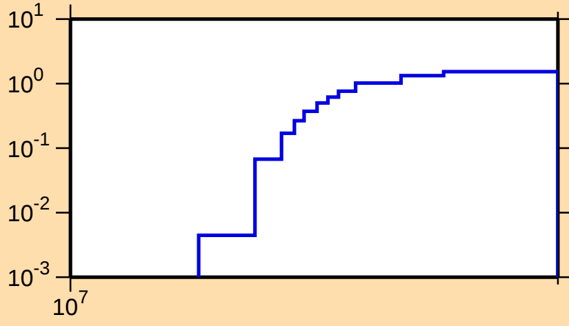
\sigma vs. E for ^{172}\text{Er}(n,3n)
