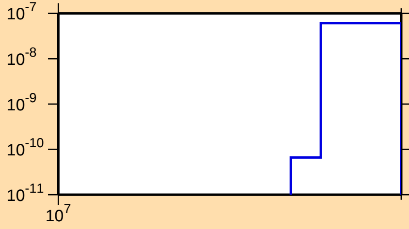
\sigma vs. E for ^{172}\text{Er}(n,nt)
