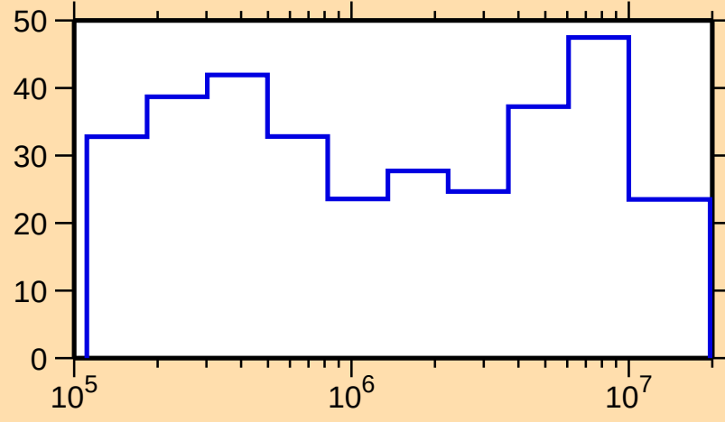
\Delta\sigma/\sigma vs. E for ^{173}\text{Er}(n,\text{el.})
