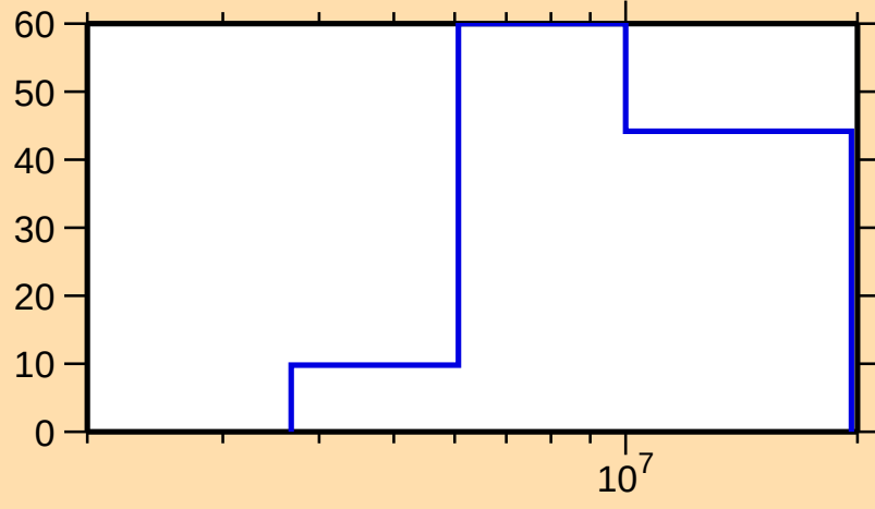
\Delta\sigma/\sigma vs. E for ^{173}\text{Er}(n,\text{inel.})
