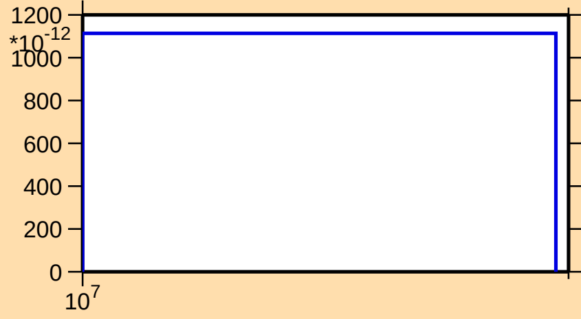
\sigma vs. E for ^{173}\text{Er}(n,2n\alpha)
