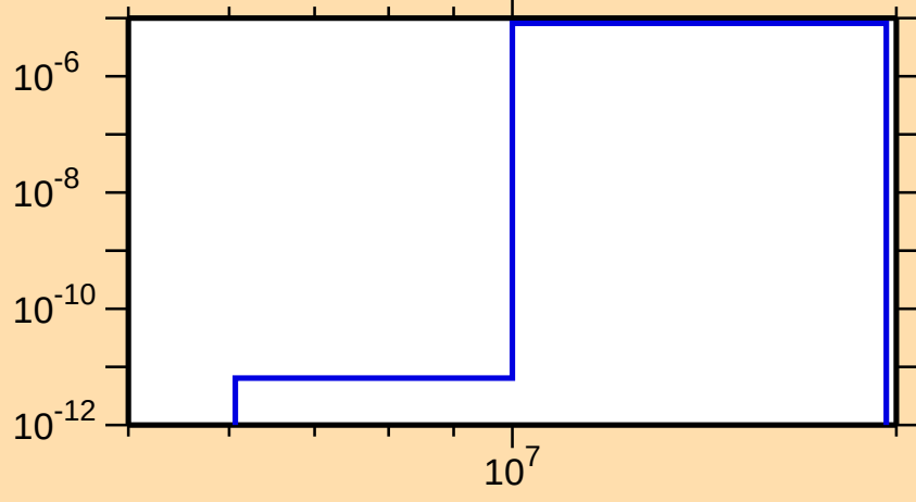
\sigma vs. E for ^{173}\text{Er}(n,n\alpha)
