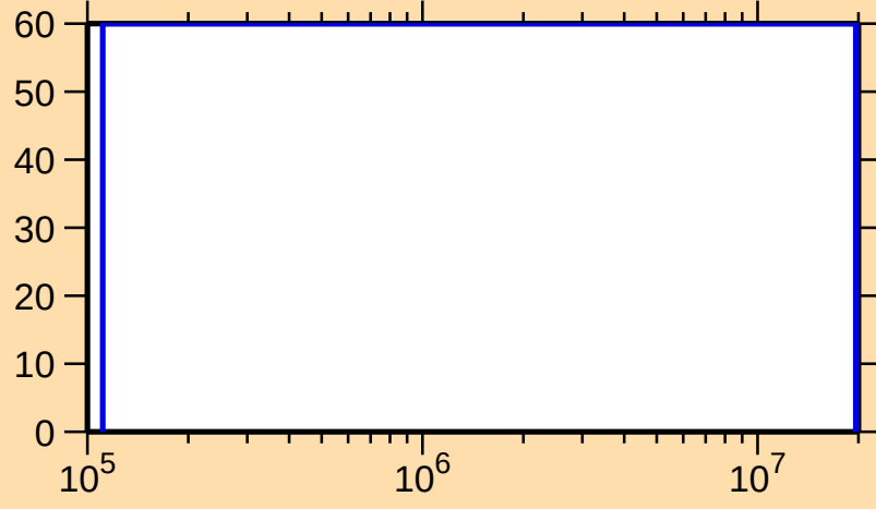
\Delta\sigma/\sigma vs. E for ^{173}\text{Er}(n,n_1)
