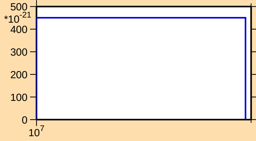
\sigma vs. E for ^{173}\text{Er}(\text{mt 11})
