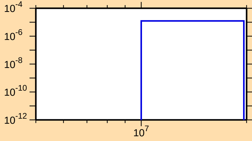
\sigma vs. E for ^{173}\text{Er}(n,t)
