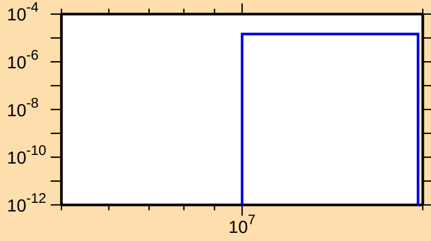
\sigma vs. E for ^{173}\text{Er}(n,np)
