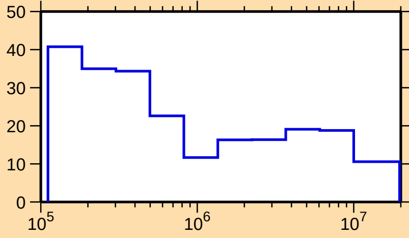
\Delta\sigma/\sigma vs. E for ^{173}\text{Er}(n,\text{tot.})
