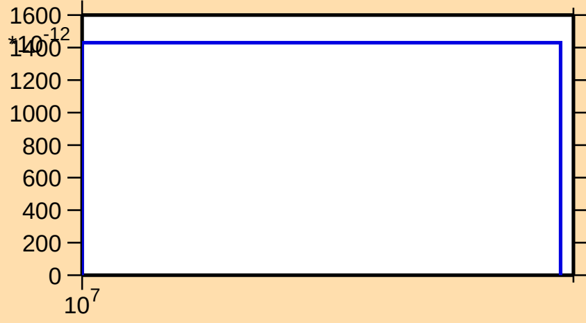
\sigma vs. E for ^{173}\text{Er}(n,nt)
