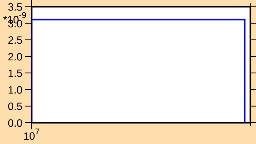
\sigma vs. E for ^{173}\text{Er}(n,\text{nd})
