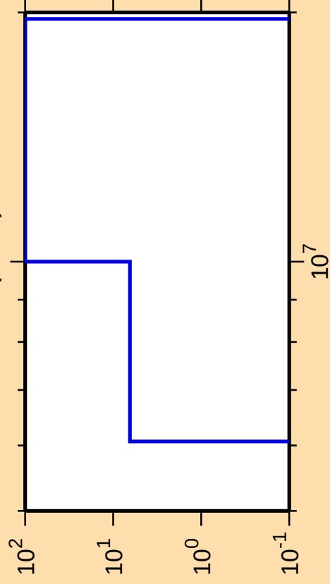
\Delta\sigma/\sigma vs. E for ^{173}\text{Er}(n,n\alpha)
