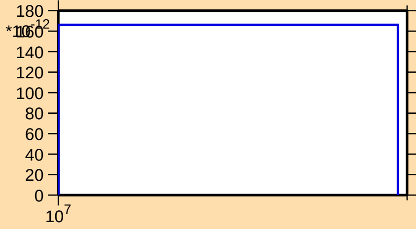
\sigma vs. E for ^{173}\text{Er}(n,2np)
