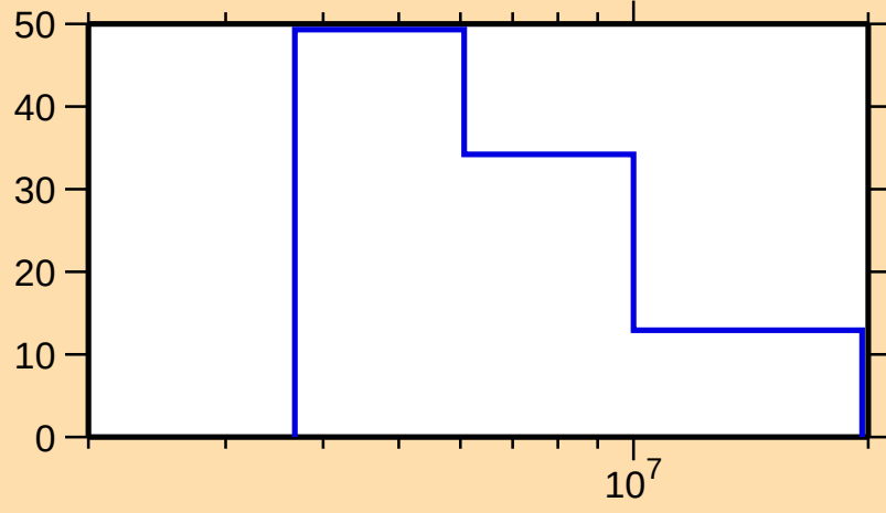
\Delta\sigma/\sigma vs. E for ^{173}\text{Er}(n,2n)
