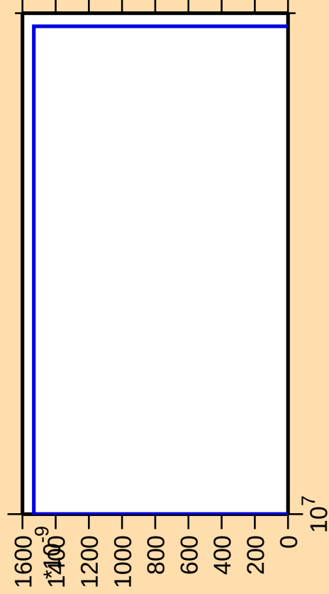
\Delta\sigma/\sigma vs. E for ^{173}\text{Er}(\text{mt 11})
