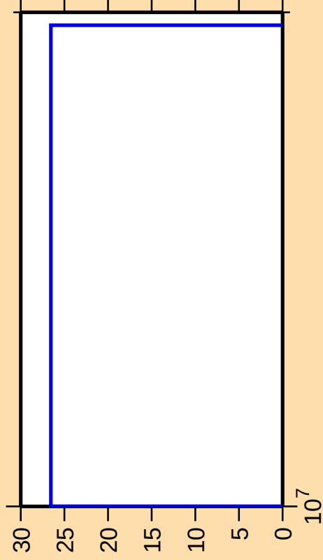
\Delta\sigma/\sigma vs. E for ^{173}\text{Er}(n,3n)
