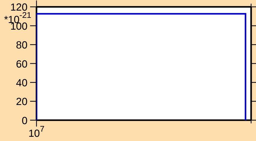
\sigma vs. E for ^{174}\text{Er}(\text{mt 11})
