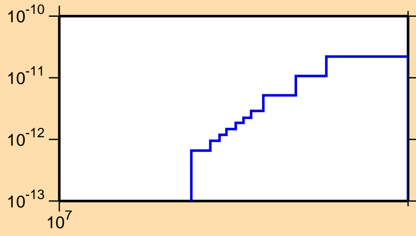
\sigma vs. E for ^{240}\text{Es} (mt 45)
