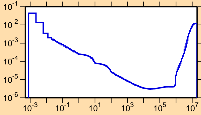
\sigma vs. E for ^{240}\text{Es}(n,p)
