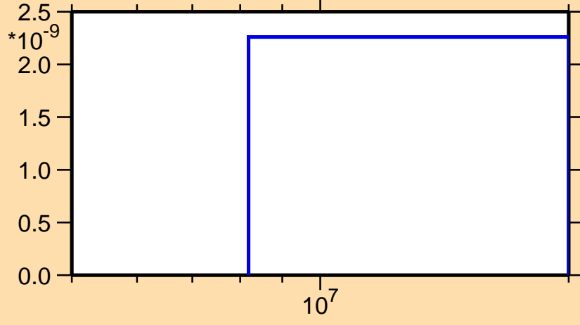
\sigma vs. E for ^{240}\text{Es}(n,nd)
