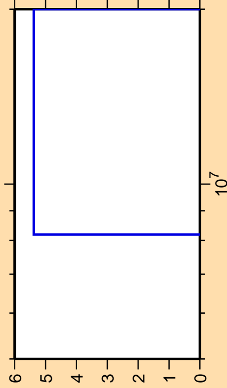
\Delta\sigma/\sigma vs. E for ^{240}\text{Es}(n,nt)
