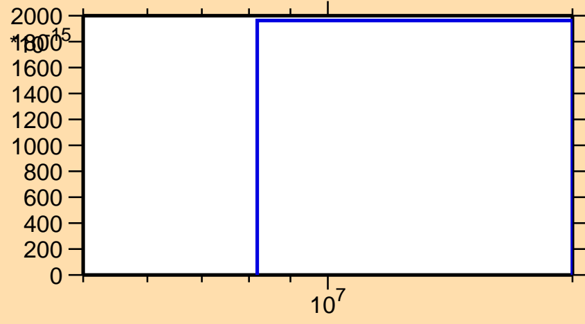
\sigma vs. E for ^{240}\text{Es} (mt 45)
