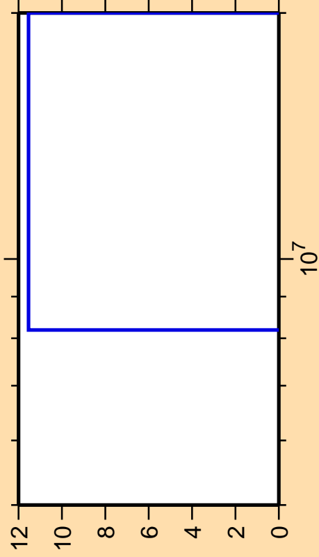
\Delta\sigma/\sigma vs. E for ^{240}\text{Es} (mt 45)
