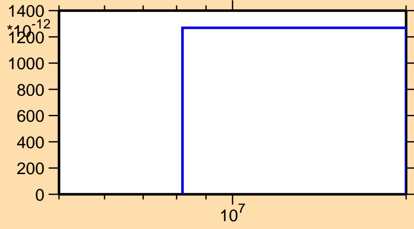
\sigma vs. E for ^{240}\text{Es}(n,3n\alpha)
