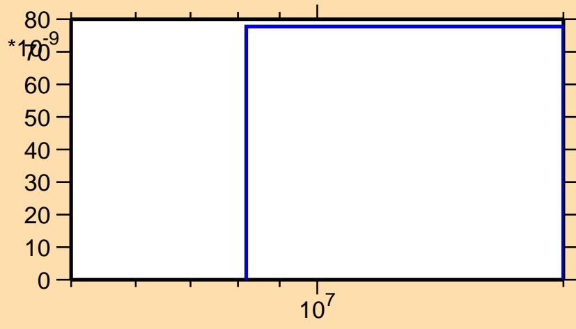
\sigma vs. E for ^{240}\text{Es}(n,\text{He3})
