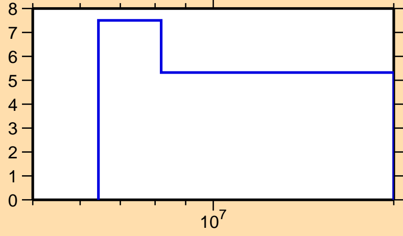
\Delta\sigma/\sigma vs. E for ^{240}\text{Es}(n,\text{nonel.})
