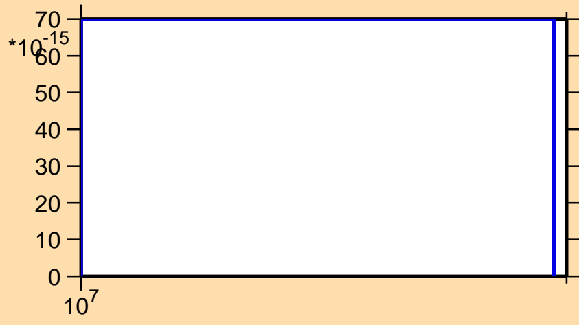
\sigma vs. E for ^{242}\text{Es}(n,pd)
