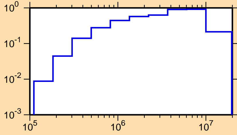
\sigma vs. E for ^{242}\text{Es}(n,\text{inel.})
