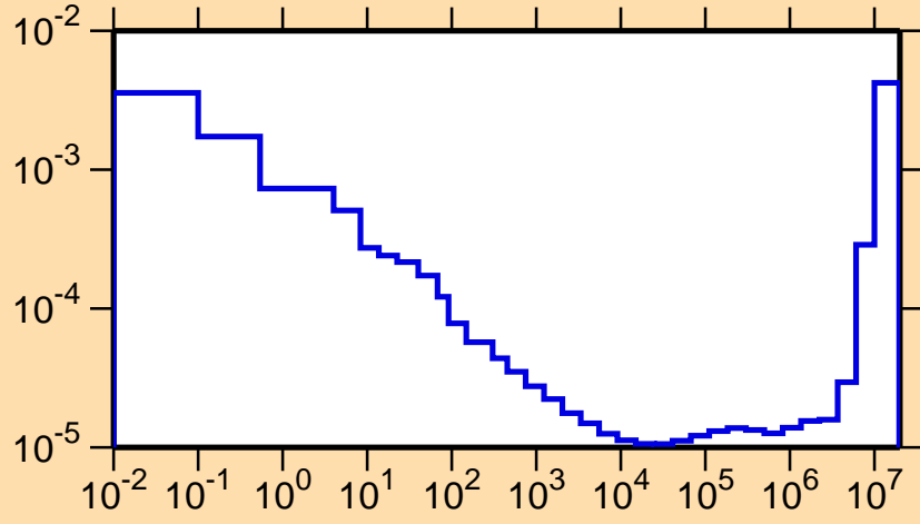
\sigma vs. E for ^{242}\text{Es}(n,\alpha)
