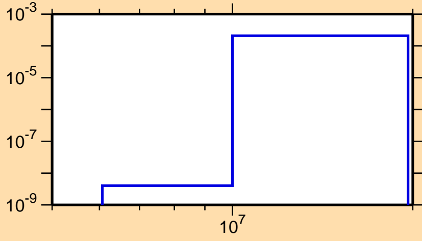
\sigma vs. E for ^{242}\text{Es}(n,t)
