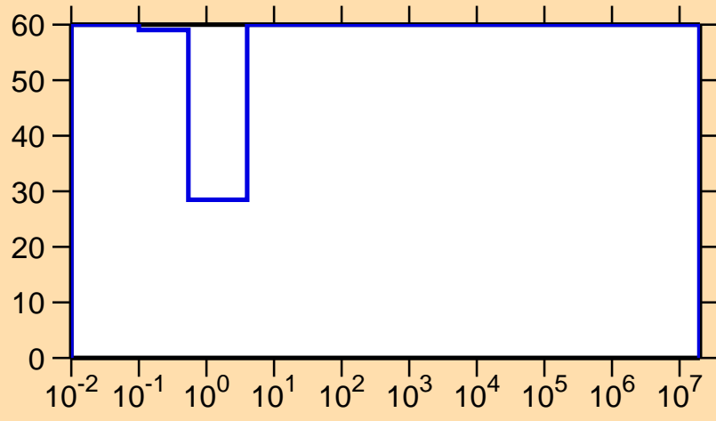
\Delta\sigma/\sigma vs. E for ^{242}\text{Es}(n,\gamma)
