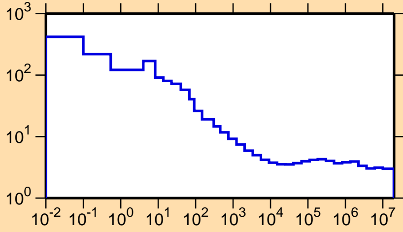
\sigma vs. E for ^{242}\text{Es}(n,\text{nonel.})
