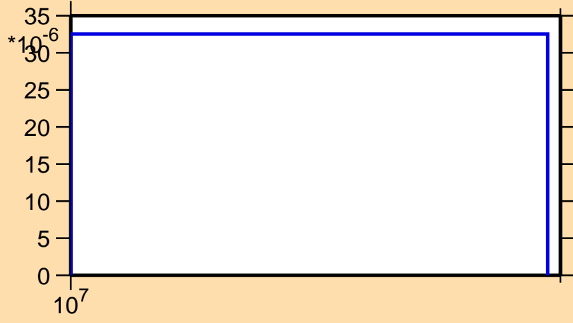
\sigma vs. E for ^{242}\text{Es}(n,3n)
