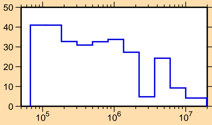
\Delta\sigma/\sigma vs. E for ^{242}\text{Es}(n,f)
