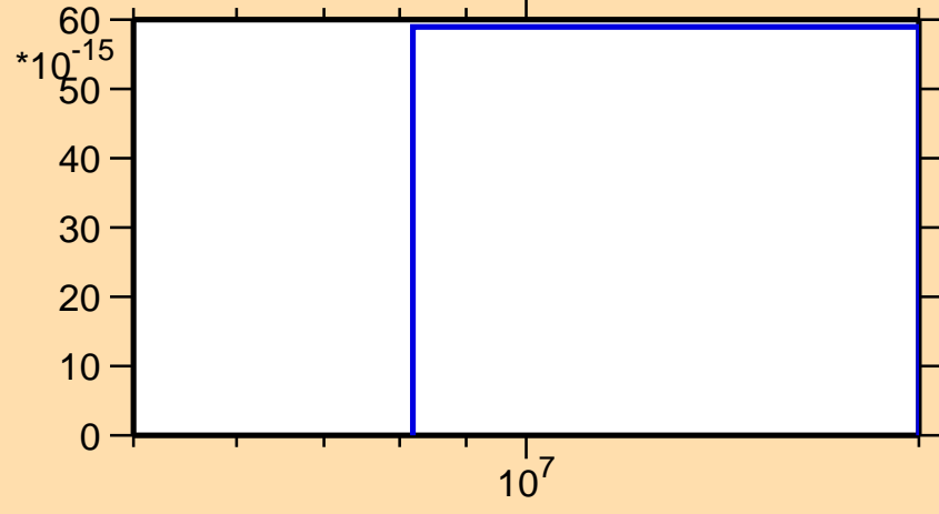
\sigma vs. E for ^{242}\text{Es}(n,pd)
