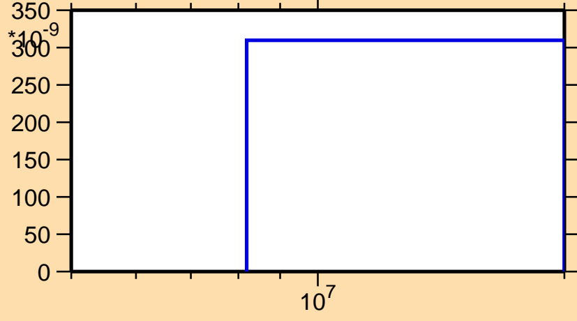
\sigma vs. E for ^{242}\text{Es}(n,2np)
