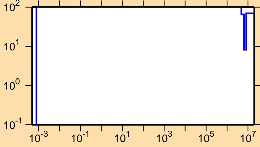
\Delta\sigma/\sigma vs. E for ^{242}\text{Es}(n,p)
