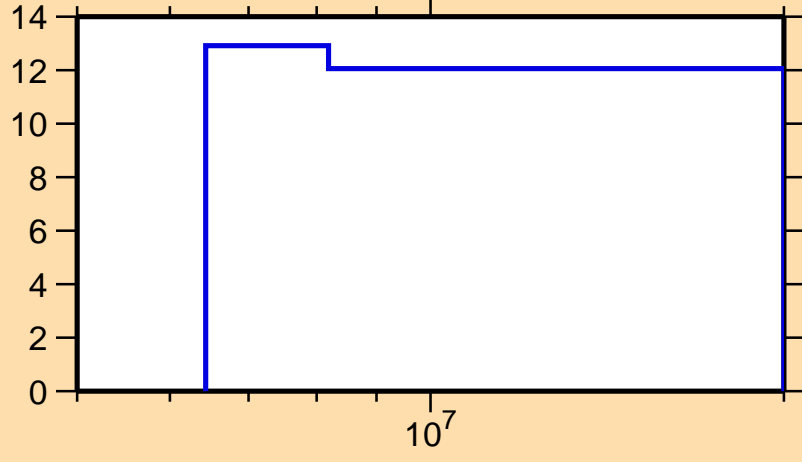
\Delta\sigma/\sigma vs. E for ^{242}\text{Es}(n,\text{tot.})
