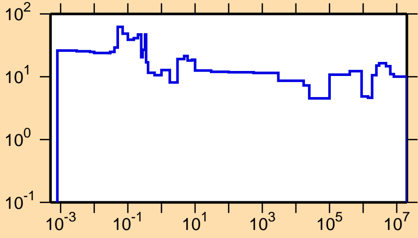
\Delta\sigma/\sigma vs. E for ^{242}\text{Es}(n,\text{el.})
