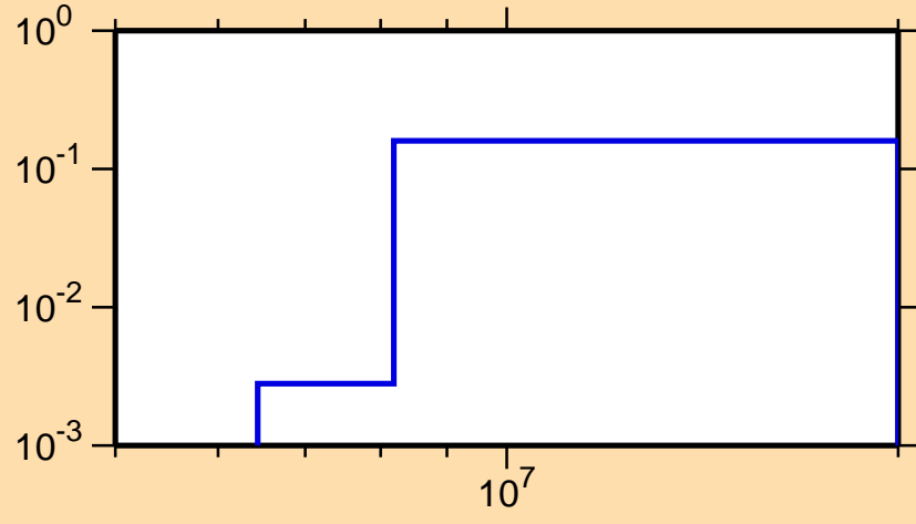
\sigma vs. E for ^{242}\text{Es}(n,2n)
