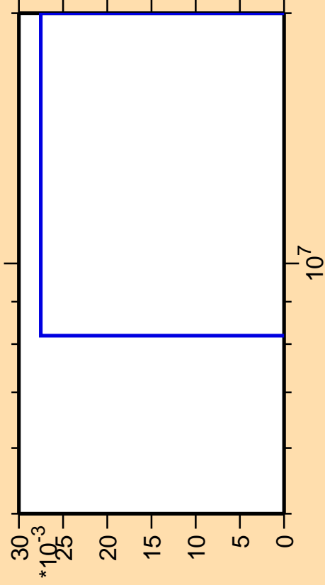
\Delta\sigma/\sigma vs. E for ^{242}\text{Es}(n,pt)
