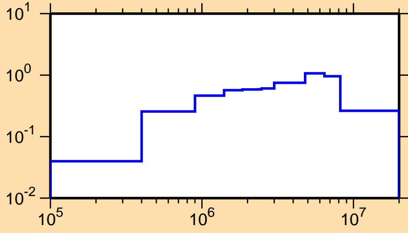
\sigma vs. E for ^{242}\text{Es}(n,n\text{cont.})
