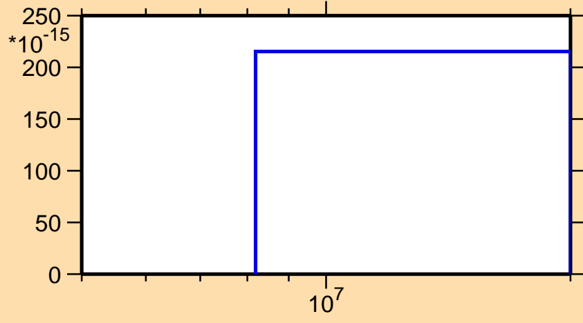
\sigma vs. E for ^{242}\text{Es}(n,3n\alpha)
