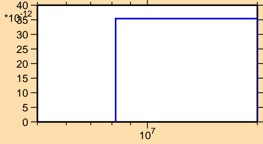
\sigma vs. E for ^{242}\text{Es}(\text{mt117})
