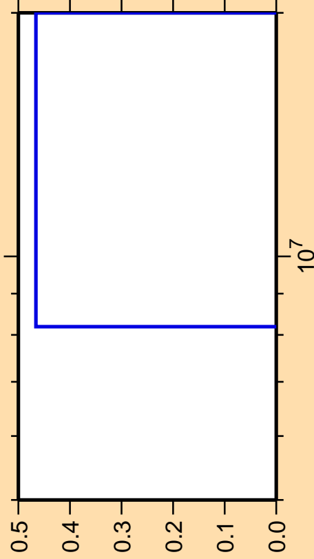
\Delta\sigma/\sigma vs. E for ^{242}\text{Es}(n,pd)
