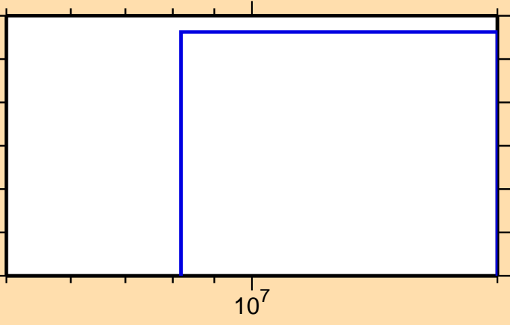
\sigma vs. E for ^{242}\text{Es}(n,nd)
