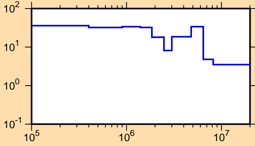
\Delta\sigma/\sigma vs. E for ^{242}\text{Es}(n,f)
