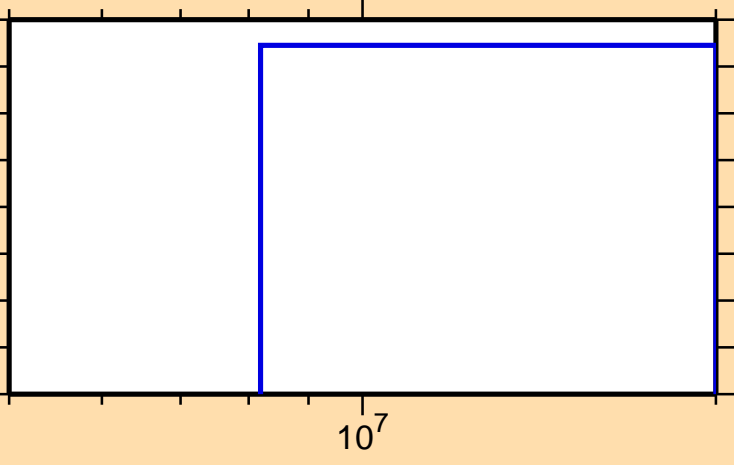
\sigma vs. E for ^{242}\text{Es}(n,\text{He3})
