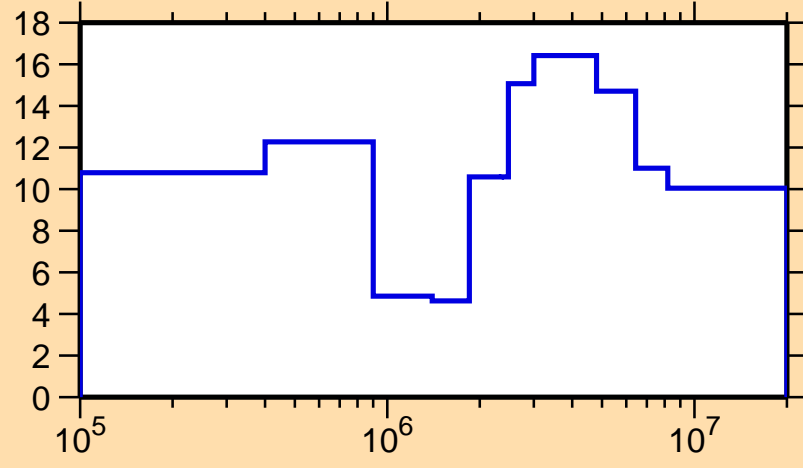
\Delta\sigma/\sigma vs. E for ^{242}\text{Es}(n,\text{el.})
