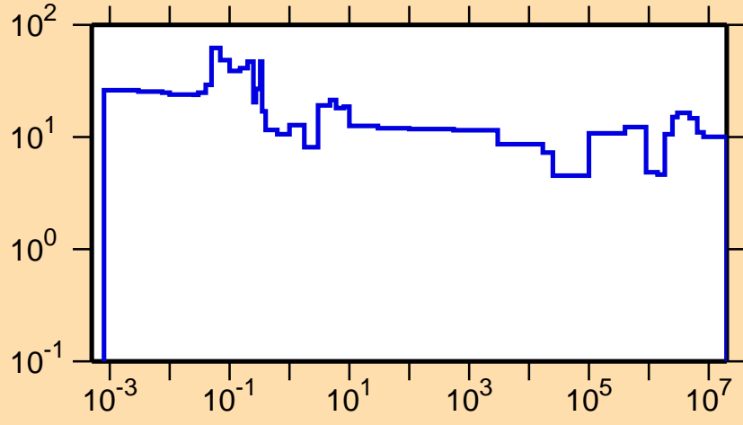
\Delta\sigma/\sigma vs. E for ^{242}\text{Es}(n,el.)
