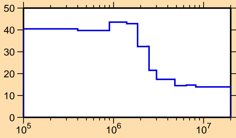
\Delta\sigma/\sigma vs. E for ^{242}\text{Es}(n,\text{nonel.})
