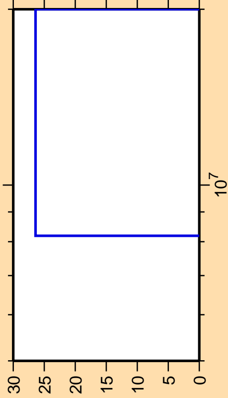
\Delta\sigma/\sigma vs. E for ^{242}\text{Es} (mt 45)
