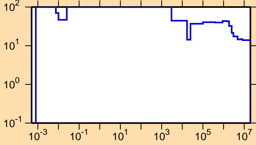
\Delta\sigma/\sigma vs. E for ^{242}\text{Es}(n,\text{nonel.})
