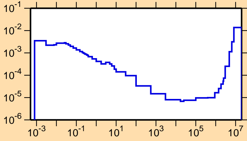
\sigma vs. E for ^{242}\text{Es}(n,p)
