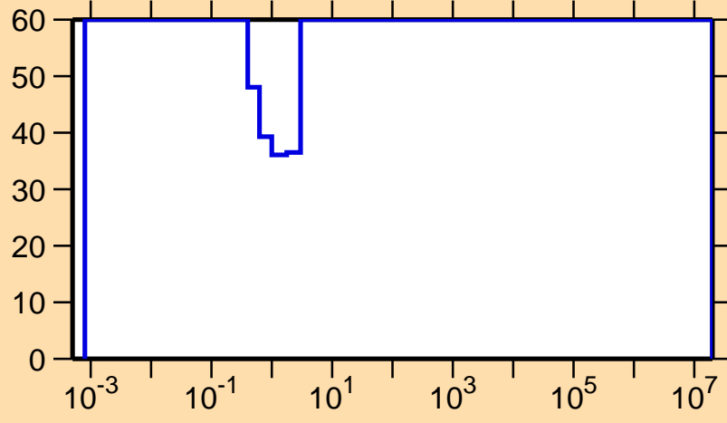
\Delta\sigma/\sigma vs. E for ^{242}\text{Es}(n,\gamma)
