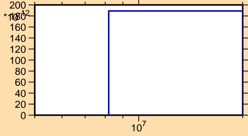
\sigma vs. E for ^{242}\text{Es}(n,nt)
