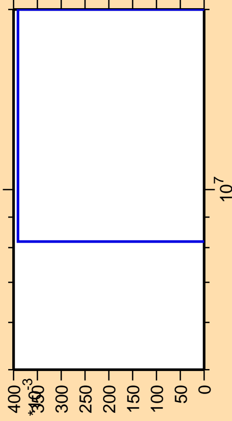
\Delta\sigma/\sigma vs. E for ^{242}\text{Es} (mt 34)
