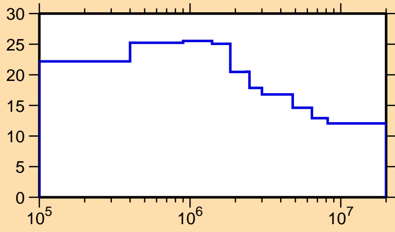
\Delta\sigma/\sigma vs. E for ^{242}\text{Es}(n,\text{tot.})
