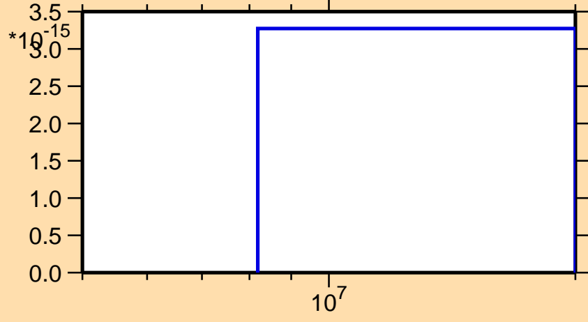
\sigma vs. E for ^{242}\text{Es}(n,pt)
