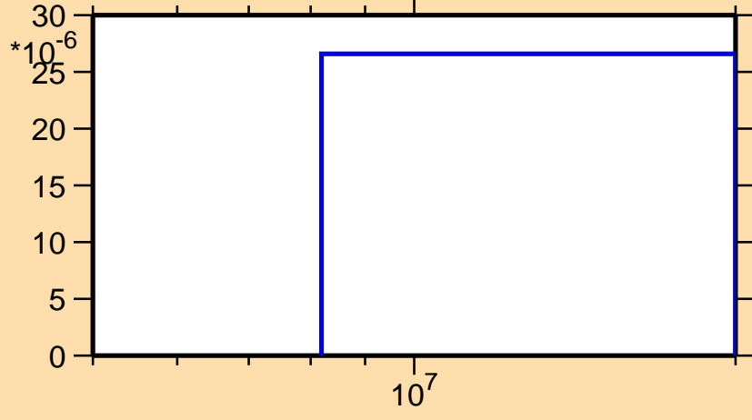
\sigma vs. E for ^{242}\text{Es}(n,3n)
