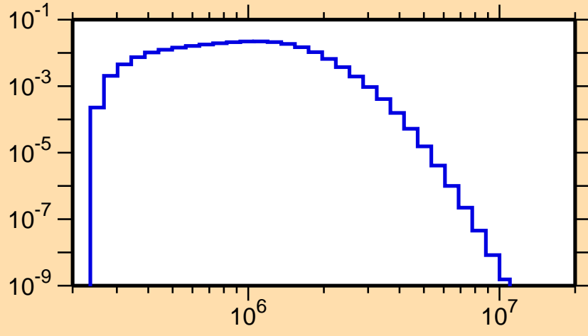
\sigma vs. E for ^{243}\text{Es}(n,n_2)
