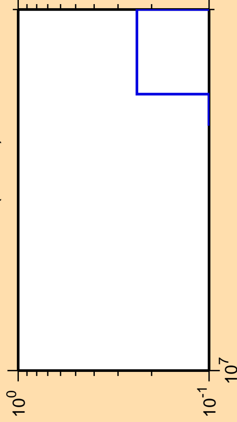
\Delta\sigma/\sigma vs. E for ^{243}\text{Es} (mt 42)
