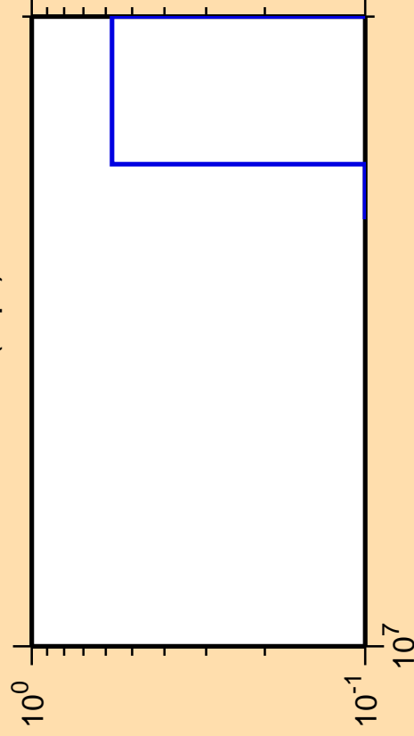
\Delta\sigma/\sigma vs. E for ^{243}\text{Es}(n,pt)
