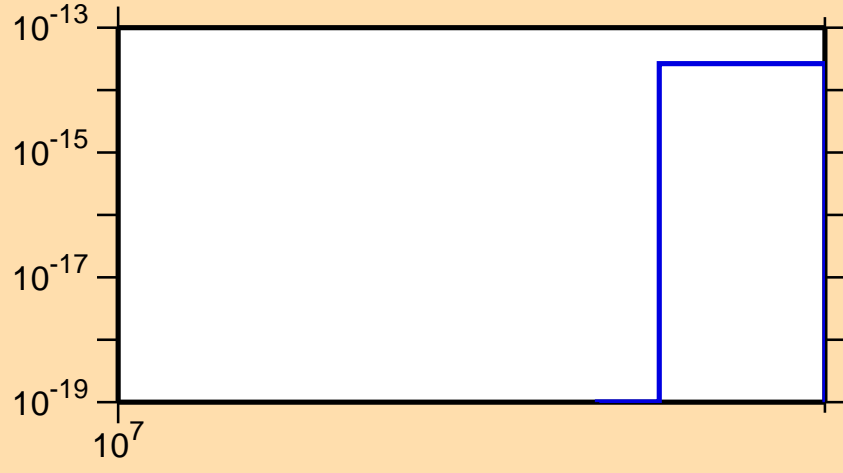
\sigma vs. E for ^{243}\text{Es} (mt 42)
