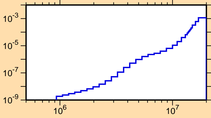
\sigma vs. E for ^{243}\text{Es}(n,n\alpha)
