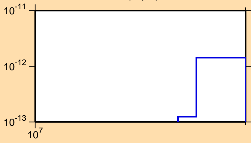
\sigma vs. E for ^{243}\text{Es}(n,pd)
