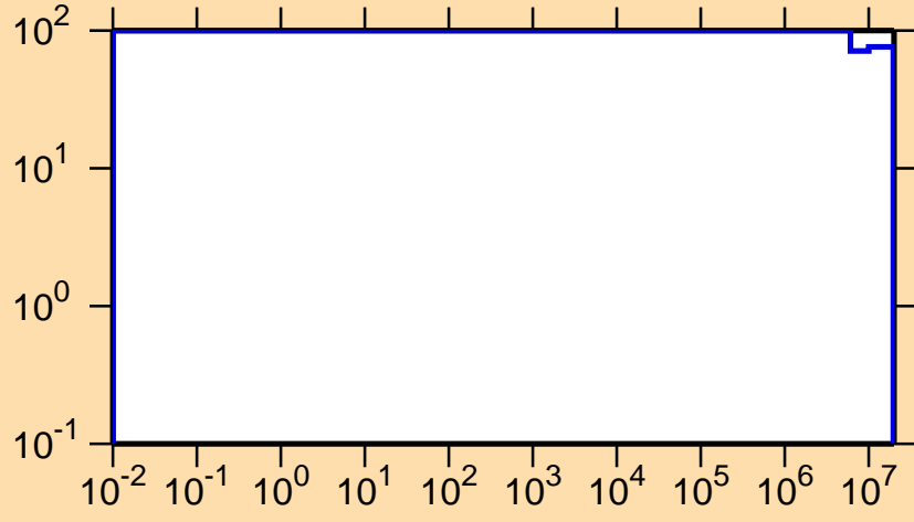
\Delta\sigma/\sigma vs. E for ^{243}\text{Es}(n,p)
