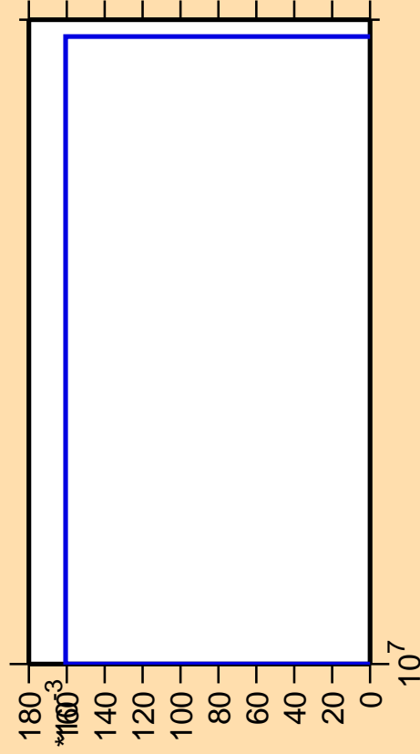
\Delta\sigma/\sigma vs. E for ^{243}\text{Es}(n,pd)
