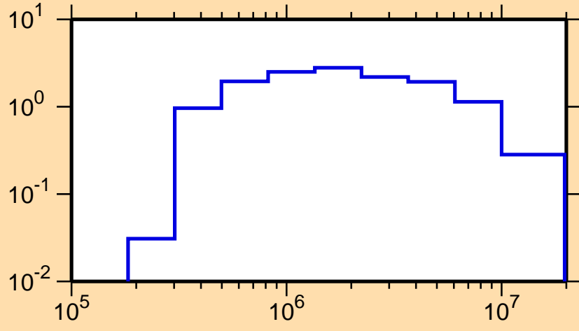
\sigma vs. E for ^{243}\text{Es}(n,\text{inel.})
