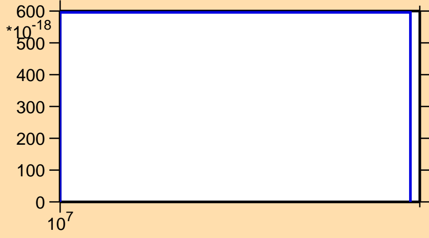
\sigma vs. E for ^{243}\text{Es}(n,pt)
