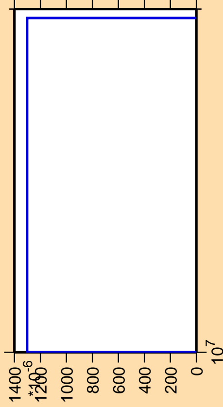
\Delta\sigma/\sigma vs. E for ^{243}\text{Es} (mt 42)
