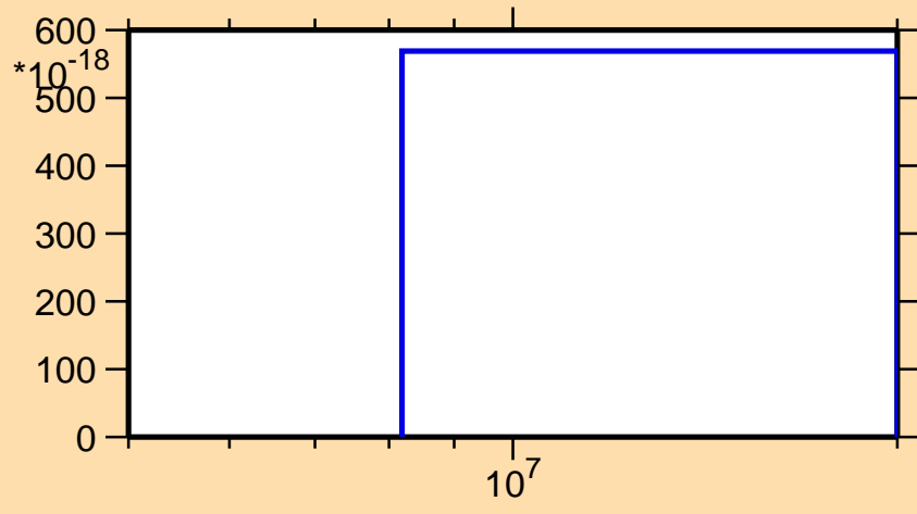
\sigma vs. E for ^{243}\text{Es}(n,pt)
