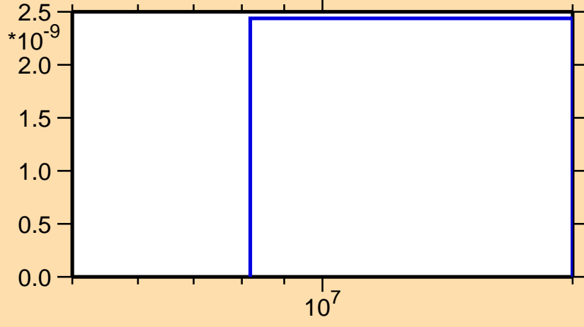
\sigma vs. E for ^{243}\text{Es}(n,nt)
