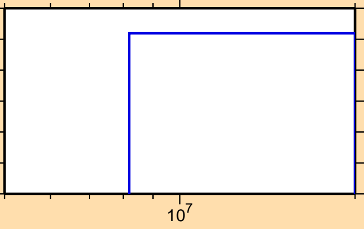
\sigma vs. E for ^{243}\text{Es}(n,\text{He3})
