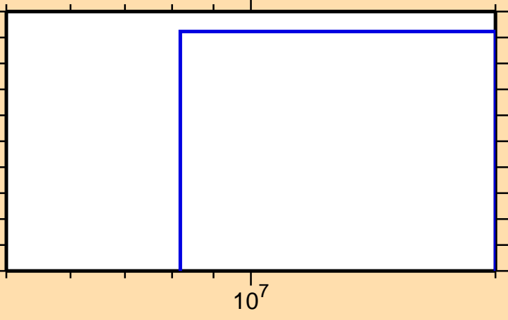
\sigma vs. E for ^{243}\text{Es}(n,pd)
