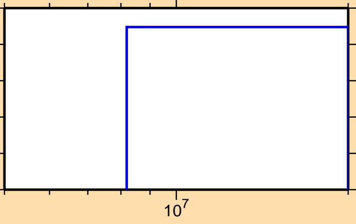
\sigma vs. E for ^{243}\text{Es}(n,2np)
