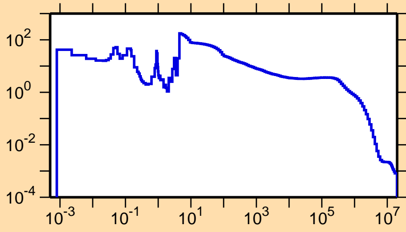
\sigma vs. E for ^{244}\text{Es}(n,\gamma)
