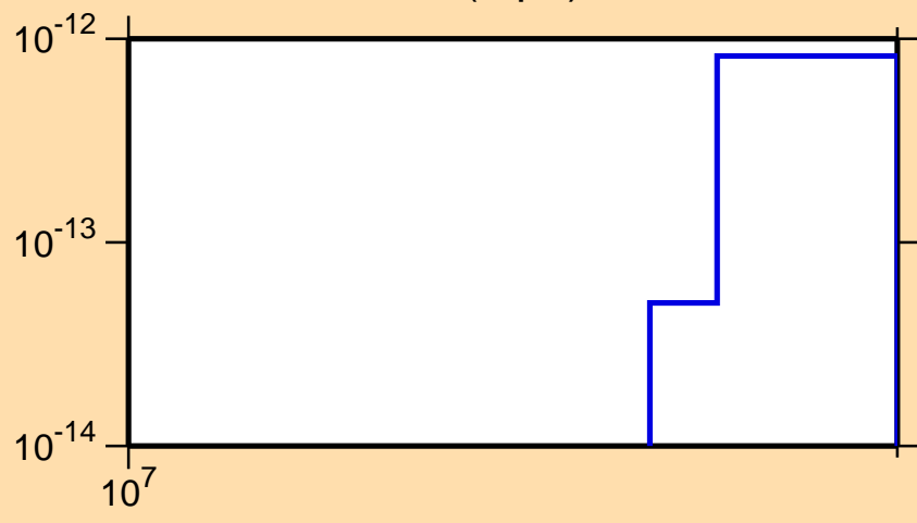
\sigma vs. E for ^{244}\text{Es}(n,pd)
