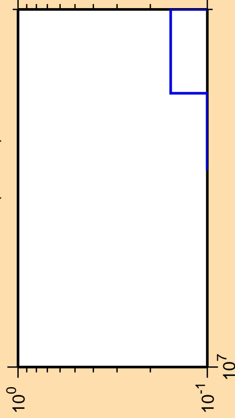
\Delta\sigma/\sigma vs. E for ^{244}\text{Es} (mt 11)
