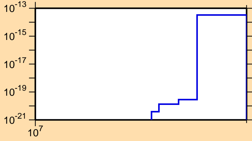
\sigma vs. E for ^{244}\text{Es} (mt 11)
