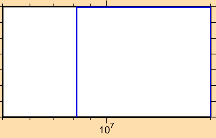
\sigma vs. E for ^{244}\text{Es}(n,nt)
