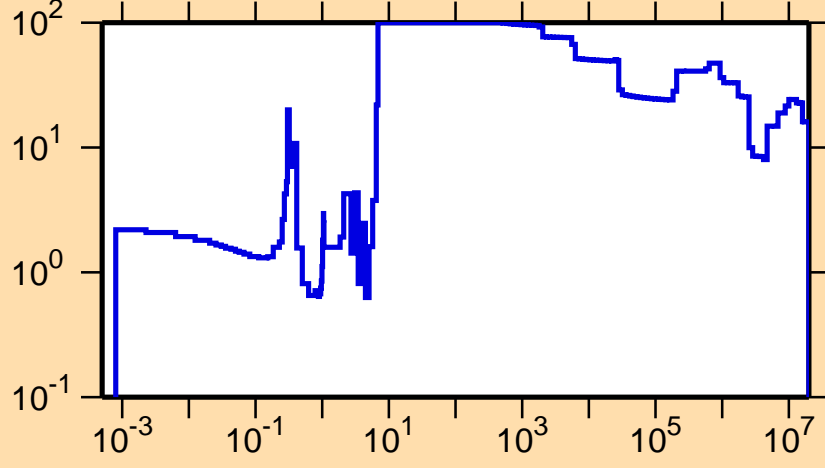
\Delta\sigma/\sigma vs. E for ^{245}\text{Es}(n,el.)
