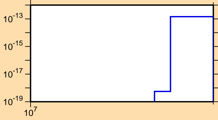
\sigma vs. E for ^{245}\text{Es} (mt 42)
