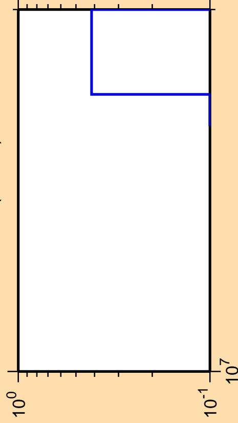
\Delta\sigma/\sigma vs. E for ^{245}\text{Es} (mt 11)
