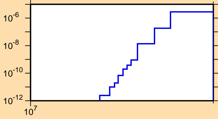
\sigma vs. E for ^{245}\text{Es}(n,nt)
