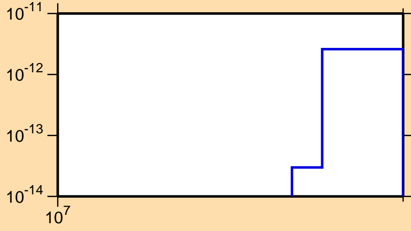
\sigma vs. E for ^{245}\text{Es} (mt 34)
