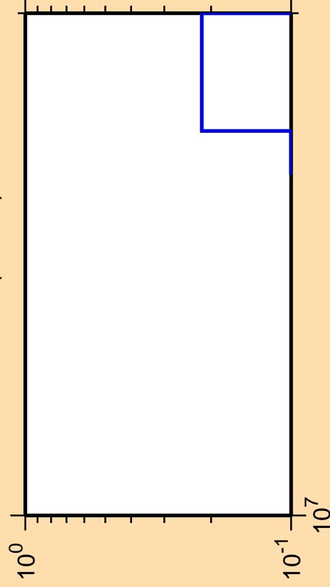
\Delta\sigma/\sigma vs. E for ^{245}\text{Es} (mt 42)
