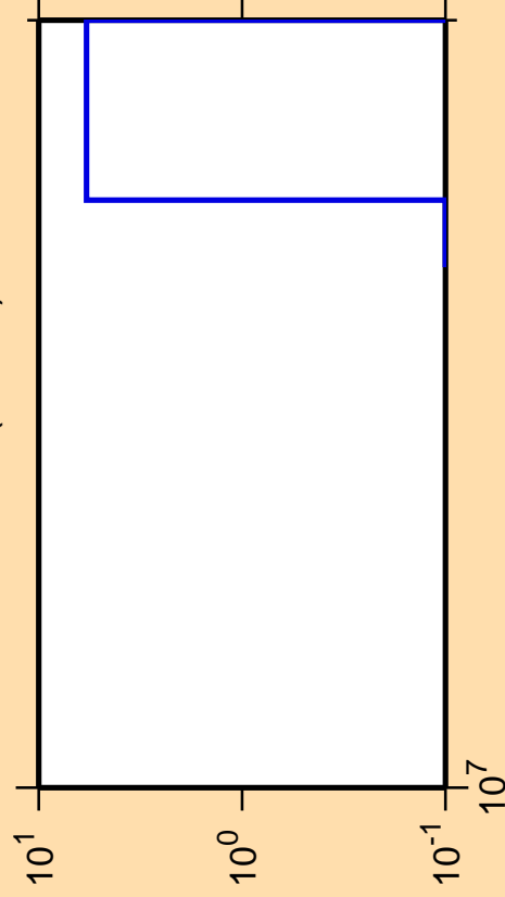
\Delta\sigma/\sigma vs. E for ^{245}\text{Es} (mt 34)
