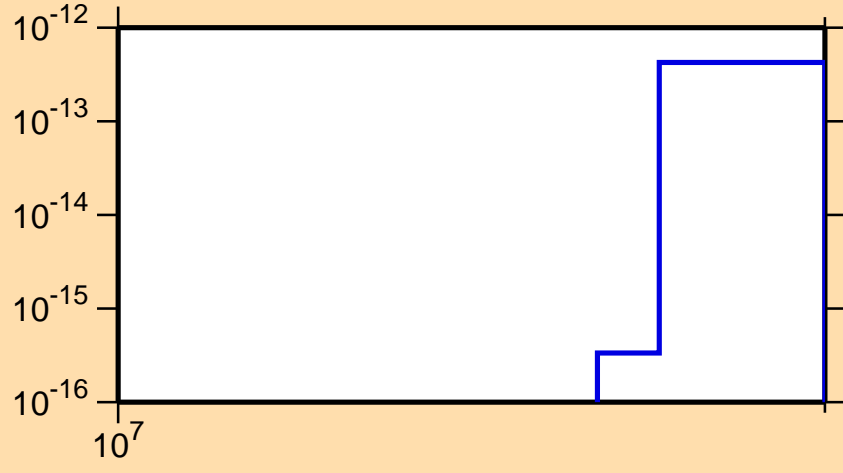
\sigma vs. E for ^{245}\text{Es} (mt 11)
