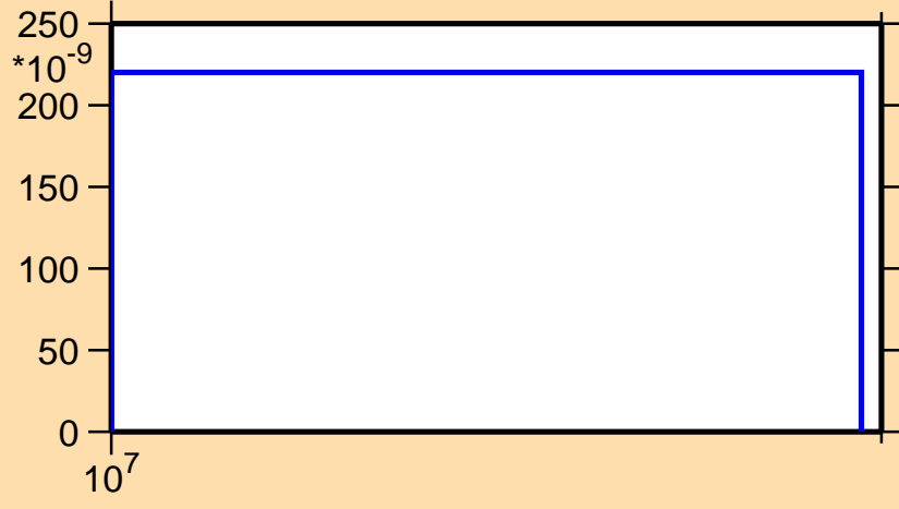
\sigma vs. E for ^{245}\text{Es}(n,2np)
