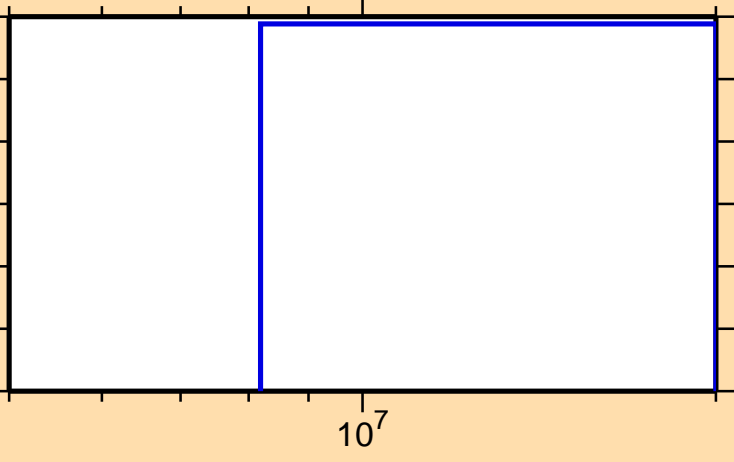
\sigma vs. E for ^{245}\text{Es}(n,nd)
