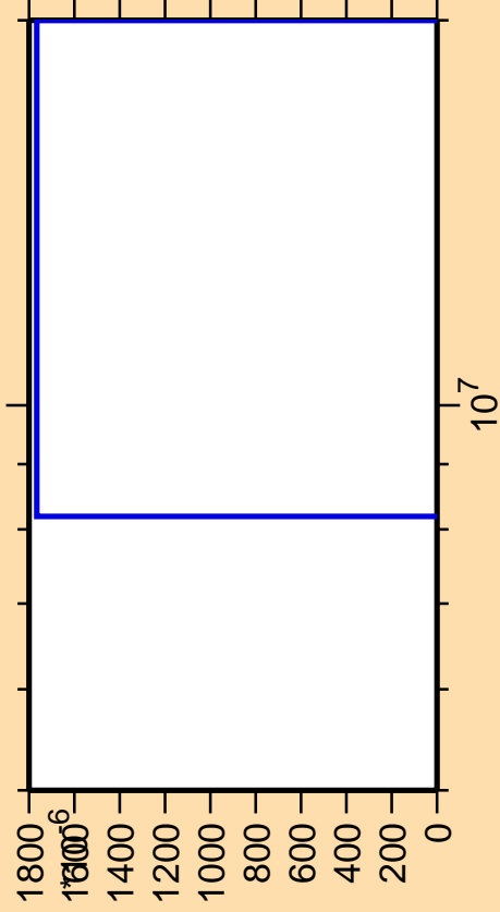
\Delta\sigma/\sigma vs. E for ^{245}\text{Es} (mt 42)
