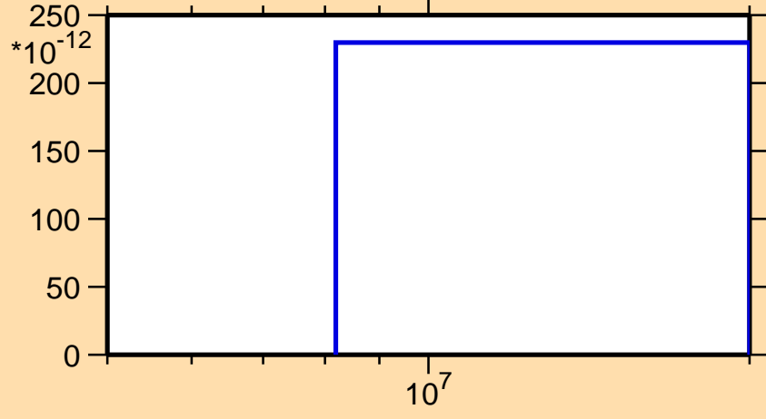
\sigma vs. E for ^{245}\text{Es}(n,p\alpha)
