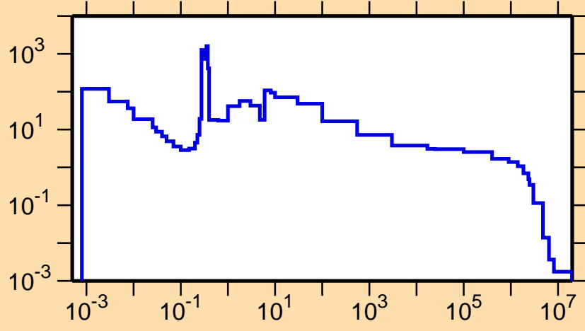
\sigma vs. E for ^{245}\text{Es}(n,\gamma)
