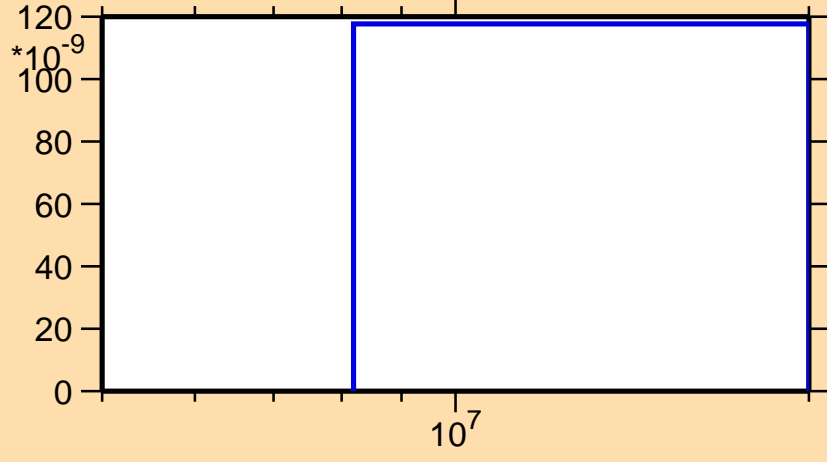
\sigma vs. E for ^{245}\text{Es}(n,nd)
