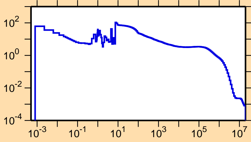
\sigma vs. E for ^{246}\text{Es}(n,\gamma)
