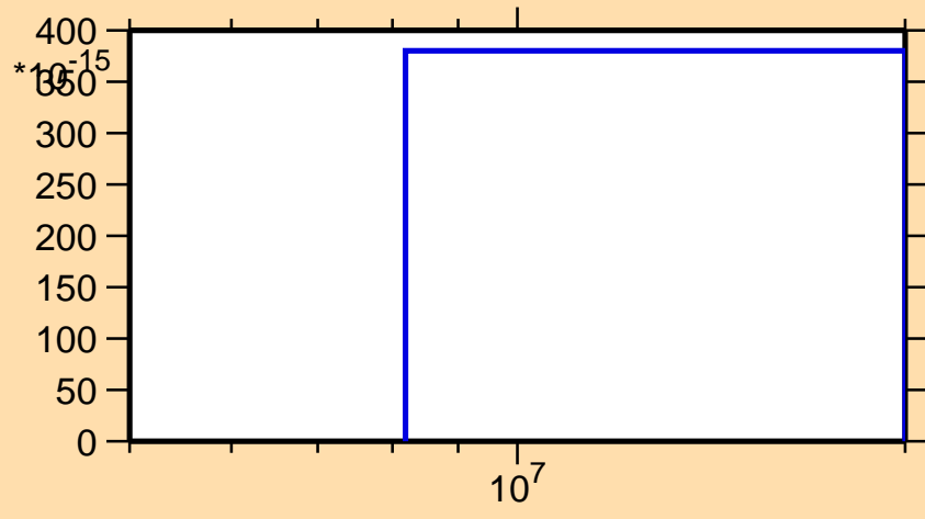
\sigma vs. E for ^{246}\text{Es} (mt 45)
