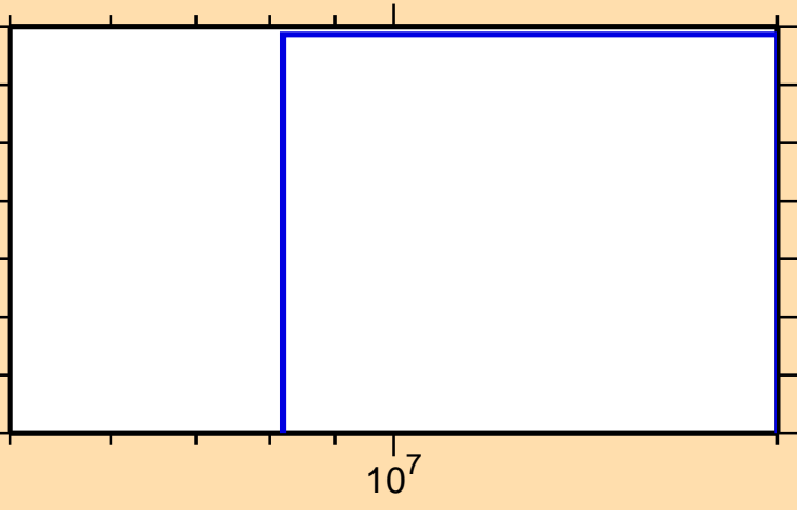
\sigma vs. E for ^{246}\text{Es}(\text{mt117})
