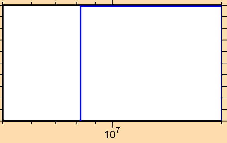
\sigma vs. E for ^{246}\text{Es}(n,\text{He3})
