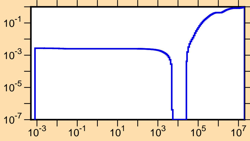
\mu vs. E for ^{247}\text{Es}(\text{mt251})
