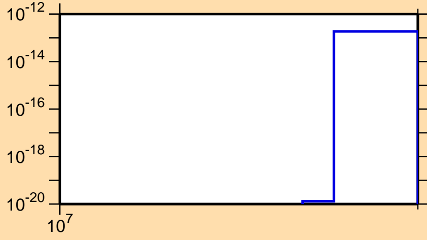
\sigma vs. E for ^{247}\text{Es} (mt 42)
