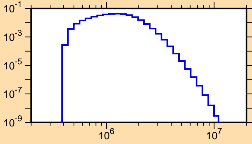
\sigma vs. E for ^{247}\text{Es}(n,n_3)
