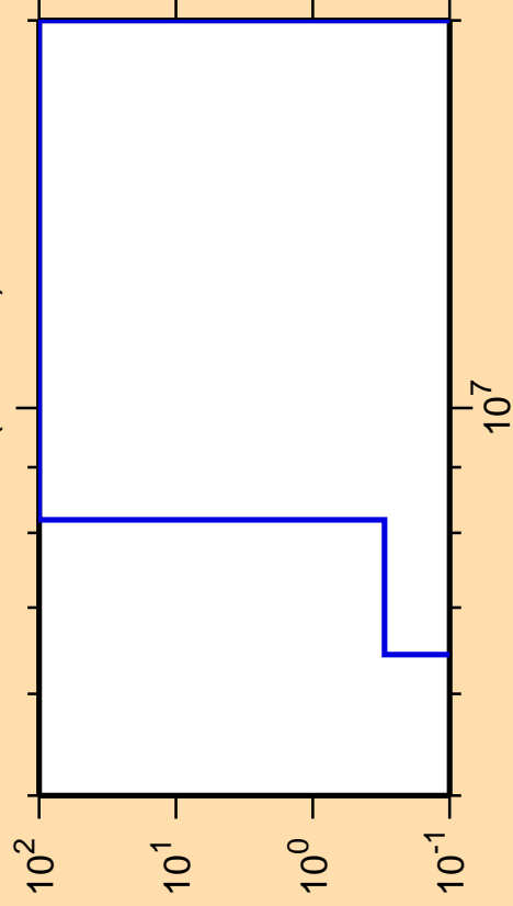
\Delta\sigma/\sigma vs. E for ^{247}\text{Es}(\text{mt117})
