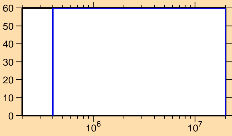
\Delta\sigma/\sigma vs. E for ^{247}\text{Es}(n,n_1)
