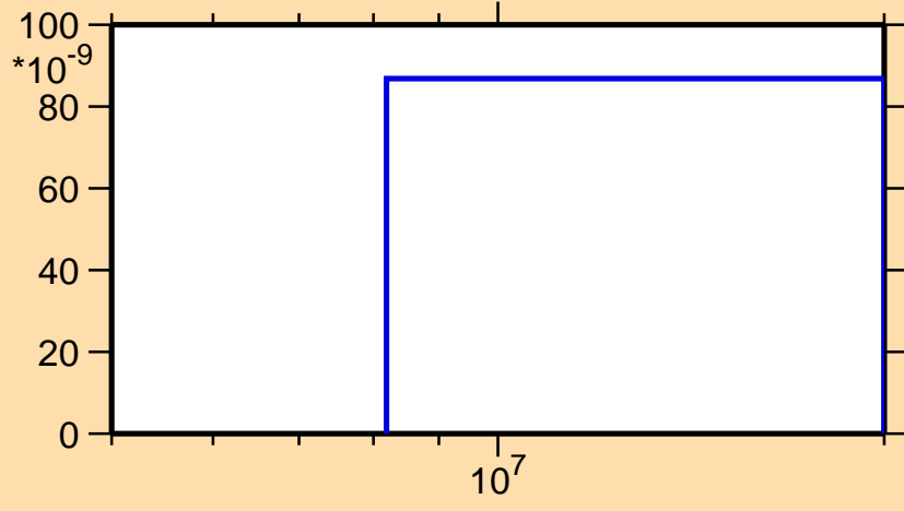
\sigma vs. E for ^{247}\text{Es}(n,nt)
