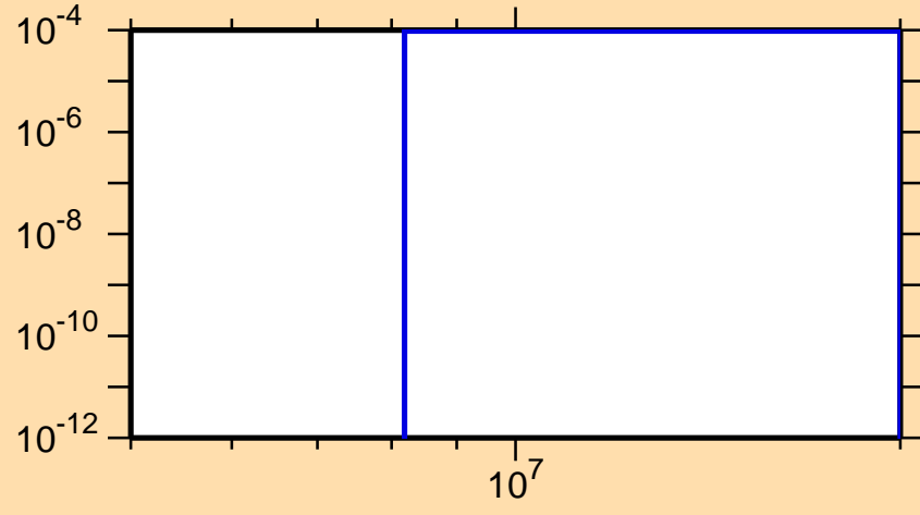
\sigma vs. E for ^{247}\text{Es}(n,t)
