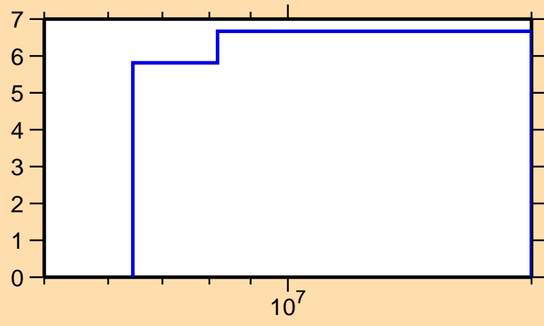
\Delta\sigma/\sigma vs. E for ^{247}\text{Es}(n,\text{nonel.})
