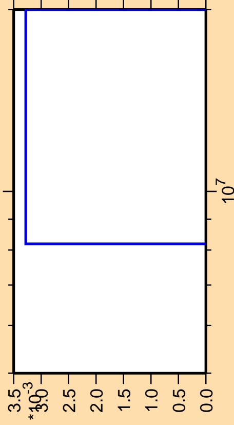
\Delta\sigma/\sigma vs. E for ^{247}\text{Es} (mt 34)
