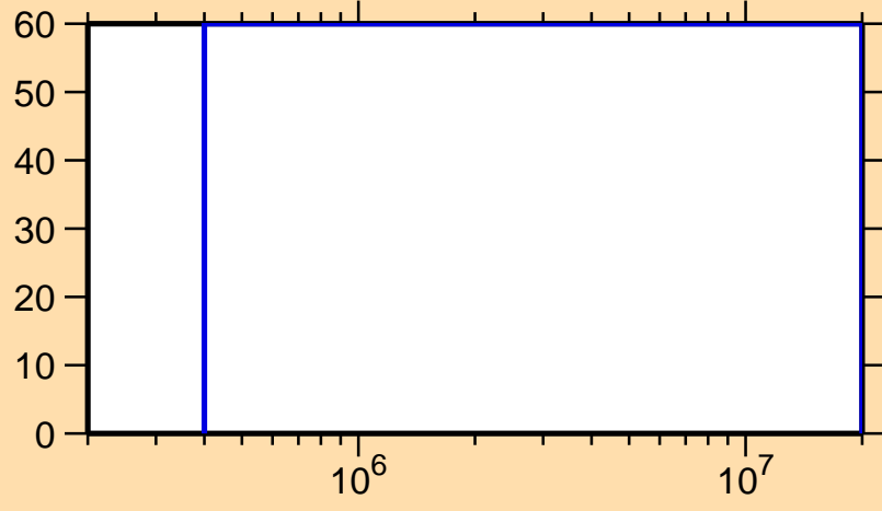
\Delta\sigma/\sigma vs. E for ^{247}\text{Es}(n,n_1)
