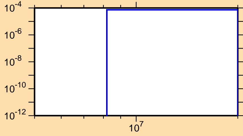
\sigma vs. E for ^{247}\text{Es}(\text{mt117})
