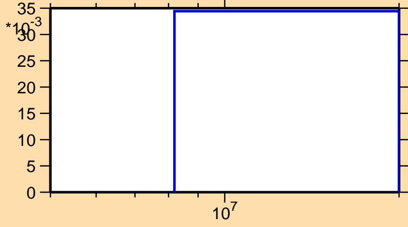
\sigma vs. E for ^{247}\text{Es}(n,3n)
