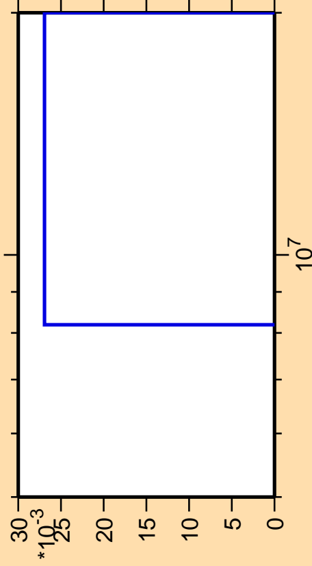
\Delta\sigma/\sigma vs. E for ^{247}\text{Es} (mt 11)
