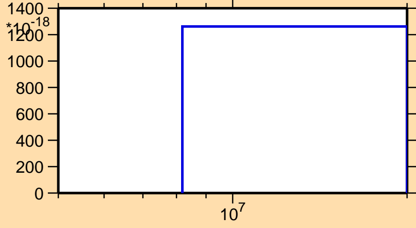
\sigma vs. E for ^{247}\text{Es} (mt 34)
