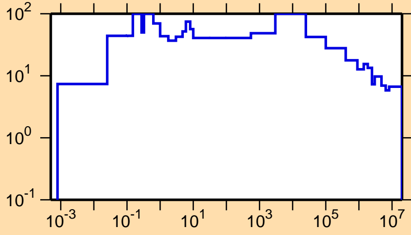
\Delta\sigma/\sigma vs. E for ^{247}\text{Es}(n,\text{nonel.})
