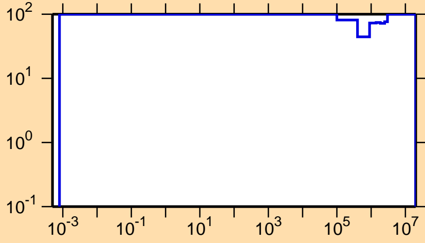
\Delta\sigma/\sigma vs. E for ^{247}\text{Es}(n,p)
