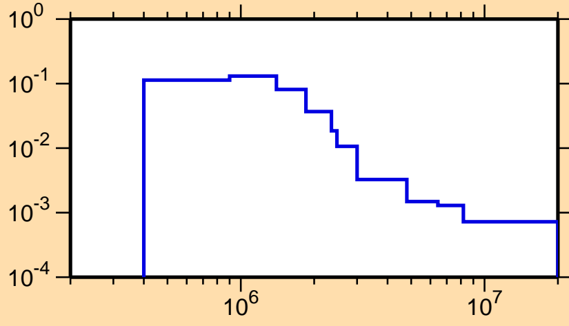
\sigma vs. E for ^{247}\text{Es}(n,n_4)
