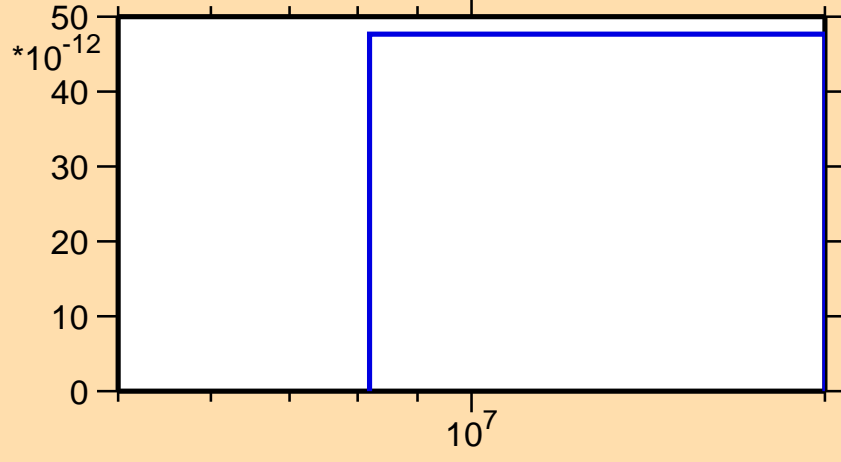
\sigma vs. E for ^{247}\text{Es}(n,p\alpha)
