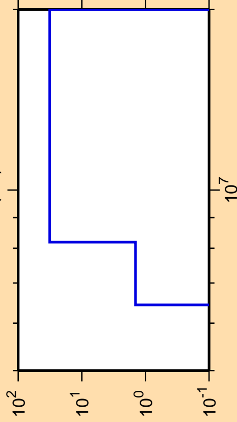
\Delta\sigma/\sigma vs. E for ^{247}\text{Es}(n,t)
