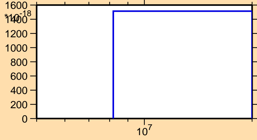
\sigma vs. E for ^{247}\text{Es} (mt 42)
