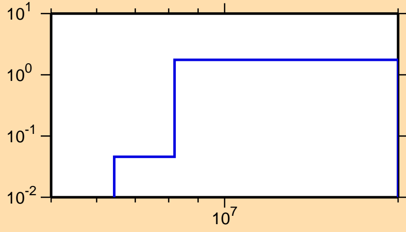
\sigma vs. E for ^{247}\text{Es}(n,2n)
