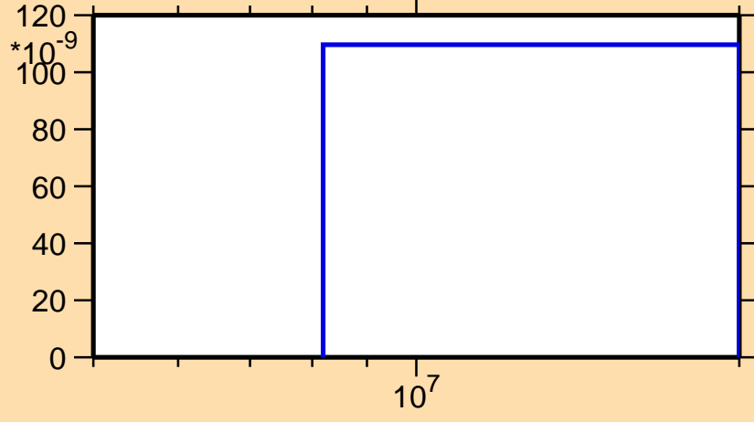
\sigma vs. E for ^{247}\text{Es}(n,2np)
