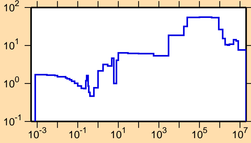
\Delta\sigma/\sigma vs. E for ^{247}\text{Es}(n,el.)
